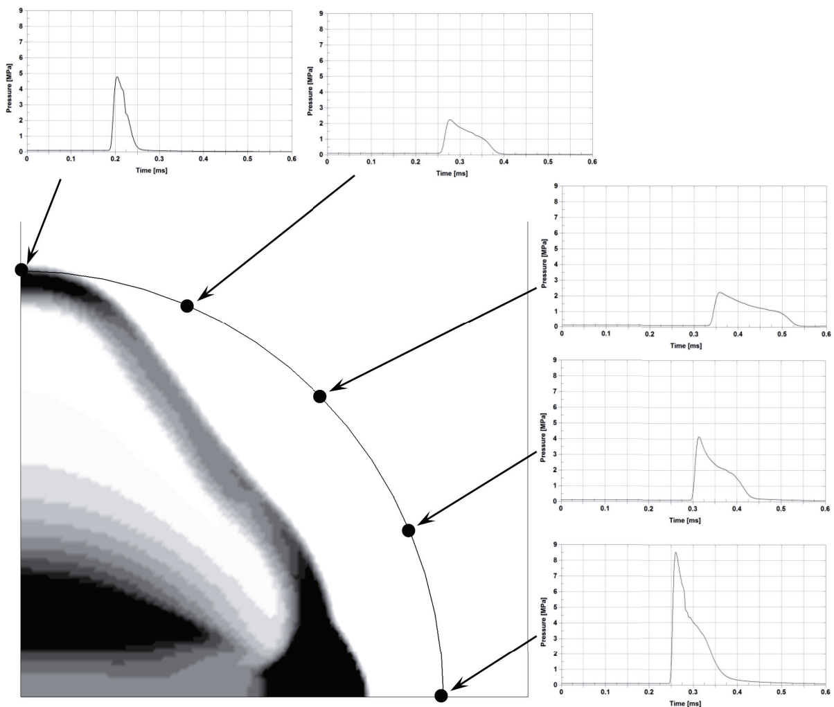
Fig. 4. The pressure history for different direction – 8 kg TNT – cylindrical shape
