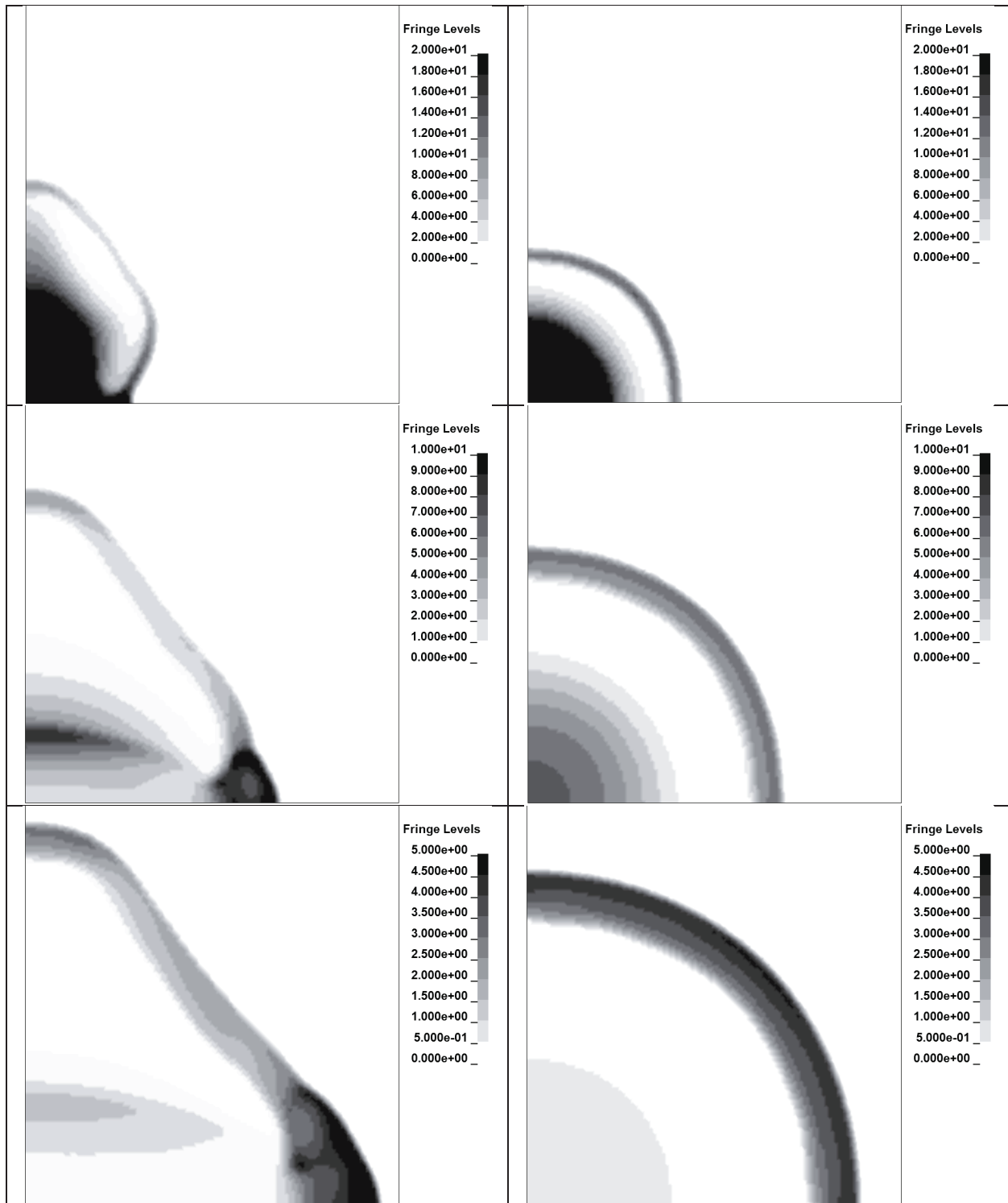
Fig. 3. Pressure wave propagation - cylindrical (left) and hemispherical shape (right) [MPa], t = 0.1; 0.2; 0.3 ms
