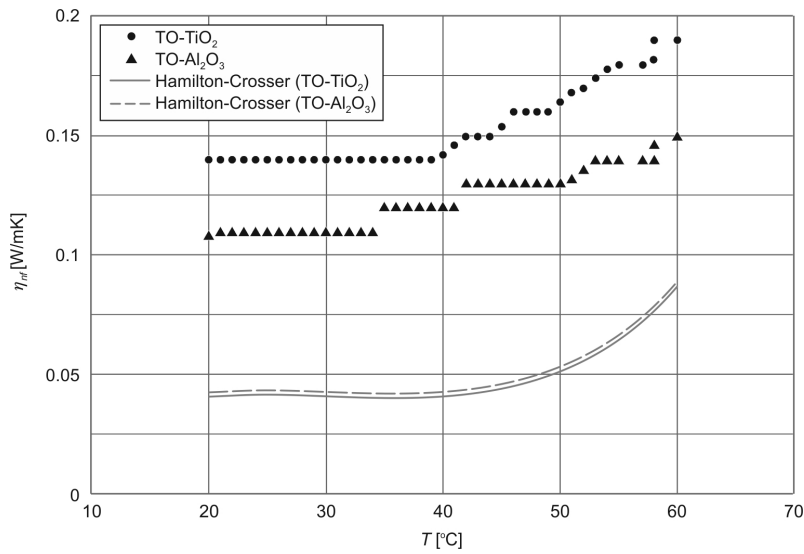
Figure 8: Comparison of the measured thermal conductivity with predictions made by use of Hamilton-Crosser's correlation, Eq. (3), for nanoparticle concentration of 5%.
