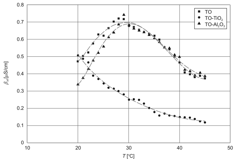
Figure 10: Electrical conductivity of TO- \text{Al}_2\text{O}_3 and TO- \text{TiO}_2 nanofluids for nanoparticle concentration of 0.1%.
