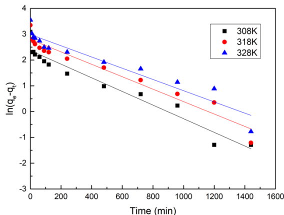
Fig. 5. Simulation of NPEO 15 adsorbing onto sub-bituminous coal by using pseudo-first order kinetics at 308, 318, and 328 K
