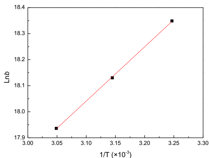
Fig. 3. Plot of \ln b vs 1/T for calculating the enthalpy change of the adsorption
