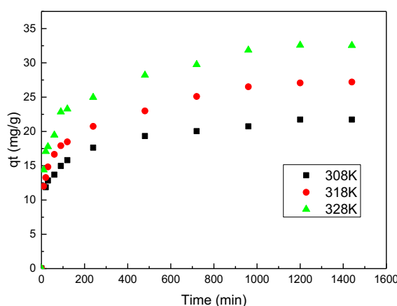
Fig. 4. Time-concentration profiles of NPEO 15 over low rank coal at 308, 318, and 328 K
