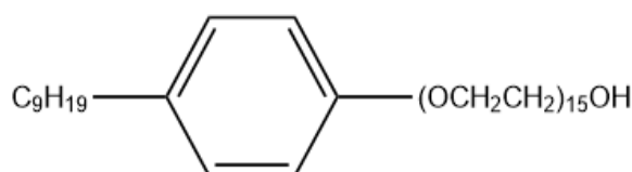
Fig. 1. Structure of NPEO 15
