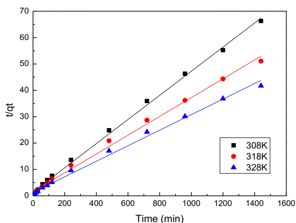
Fig. 6. Simulation of NPEO 15 adsorbing onto sub-bituminous coal by using pseudo-second order kinetics at 308, 318, and 328 K
