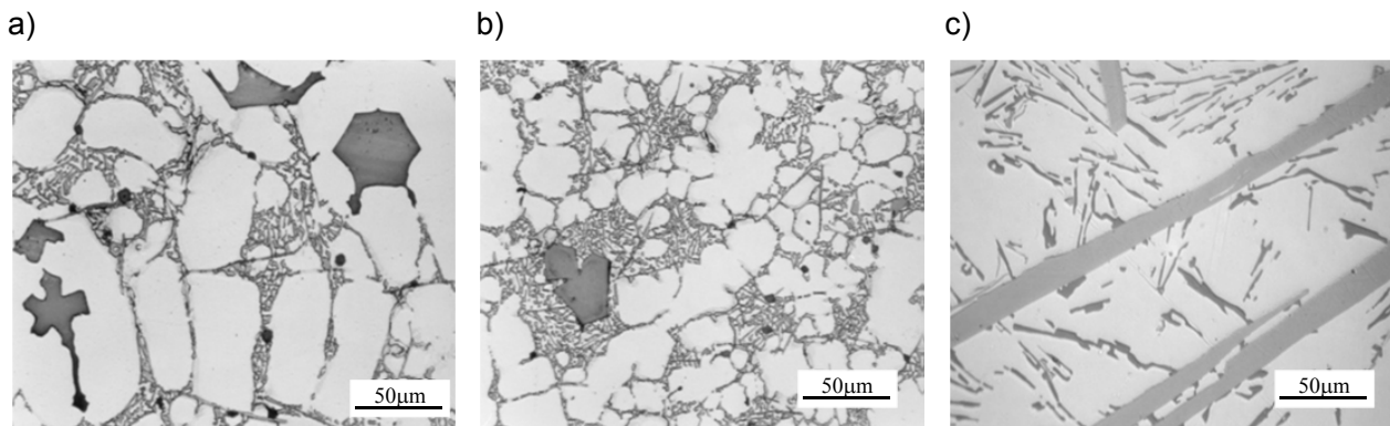
Fig. 1. Primary precipitates of the AlFeMnSi phases, microstructure of the technical AlSi alloys, LM: a) cast part in sand mould, alloy AlSi9Cu, b) cast part in metal mould, alloy AlSi9Cu, c) cast part in sand mould, alloy AlSi11FeMn
