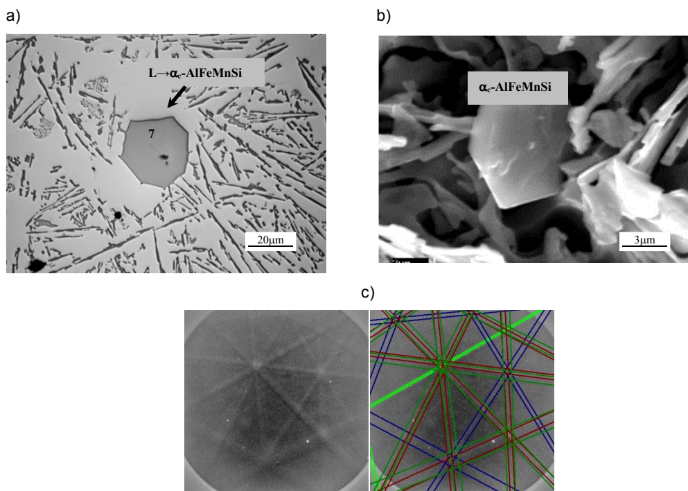
Fig. 9. Microstructure of the AlFe3.0Mn2.0Si11 alloy, cooling rate 3 K/min; pre-eutectic equiaxed polyhedron of the \alpha_c -AlFeMnSi phase: a) LM and b) SEM, c) EBS diffraction pattern, reference cubic phase: Al4.01MnSi0.74 CI 0.108 (point 7, Fig. 9a)
