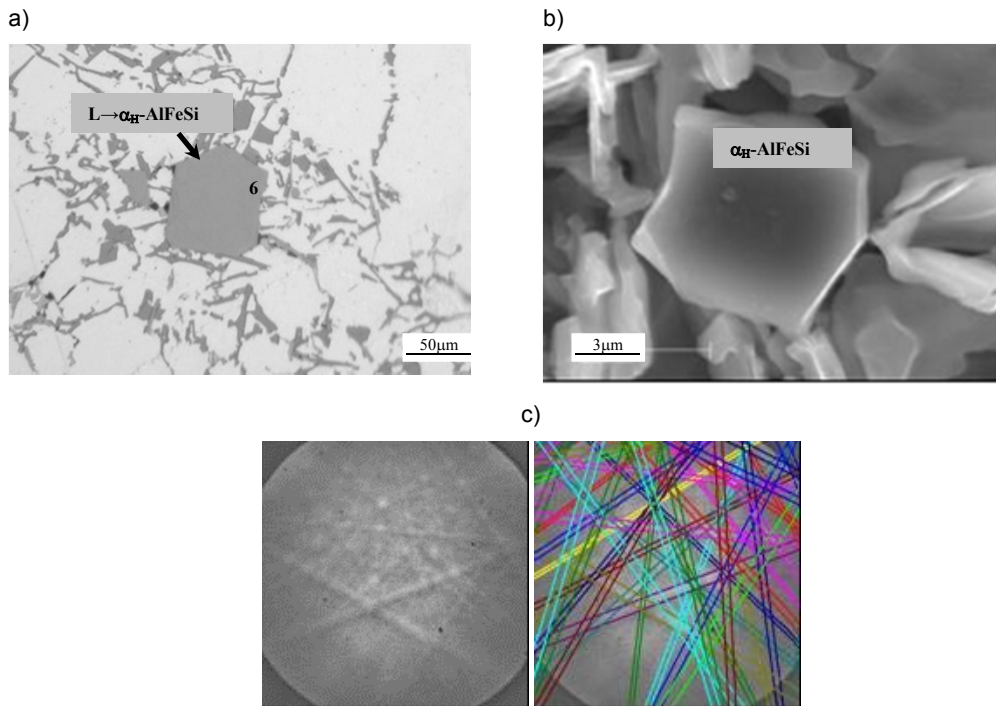
Fig. 8. Microstructure of the AlFe3.0Mn0.5Si11 alloy, cooling rate 3 K/min, pre-eutectic particle of the \alpha_H -AlFeSi phase: a) LM, b) SEM and c) EBS diffraction pattern (point 6, Fig. 8a), reference hexagonal phase: Al8Fe2Si, CI 0.52
