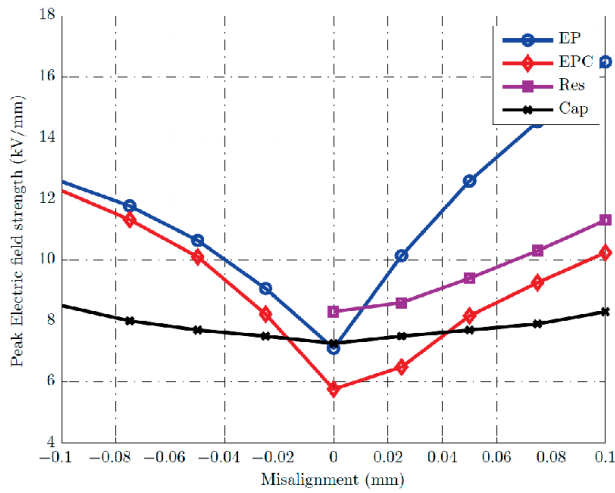
Fig. 15. Peak electric field strength for electrode profiling (EP), resistive (Res), capacitive (Cap) and the combined field control method (EPC) for different amplitudes of misalignment
