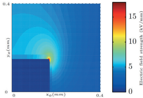
Fig. 8. Electric field distribution of the linear motor configuration without field control method
