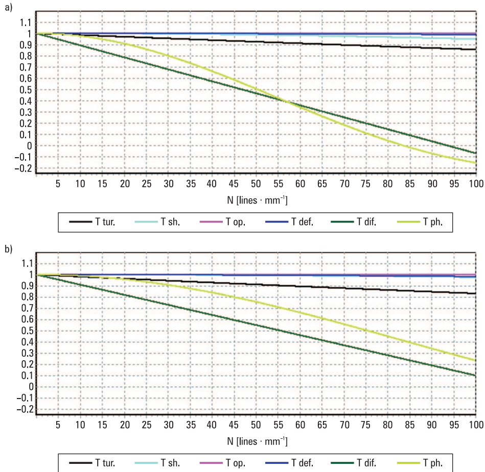
Fig. 2. Modulation transfer functions for different factors: a) for the Ikonos-2 system, b) for the WorldView-2 system
