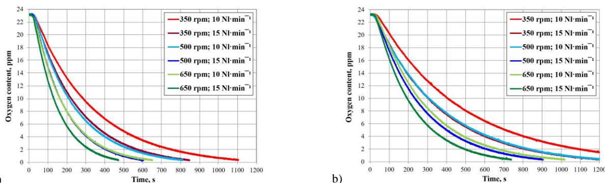
Fig. 4. Influence of the change of volume flow rate of inert gas and rotary impeller speeds on the concentration of oxygen for the individual impellers: (a) F2A 190, (b) J8 190 [10]
