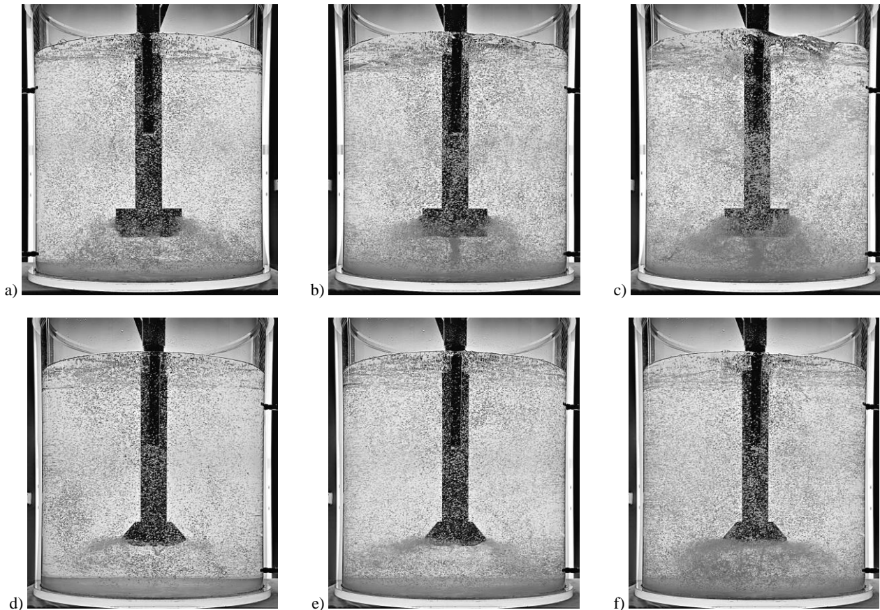
Fig. 7. Visualization images of the flow of gas in the bath at the volume flow rate of inert gas of 10 \text{Nl}\cdot\text{min}^{-1} : (a) F2A 190 – 350 rpm, (b) F2A 190 – 500 rpm, (c) F2A 190 – 650 rpm, (d) J8 190 – 350 rpm, (e) J8 190 – 500 rpm, (f) J8 190 – 650 rpm [10]
