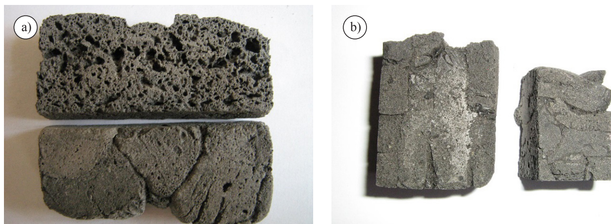
Fig. 4. Illustration of fragments of thermal insulation zones sections in complicated form structures performed by the working zone filling with fragmented elements and the subsequent heat treatment in dismantable equipment of varying complexity: a) - without limiting the free volume of formation; b) - with restriction of formation space
