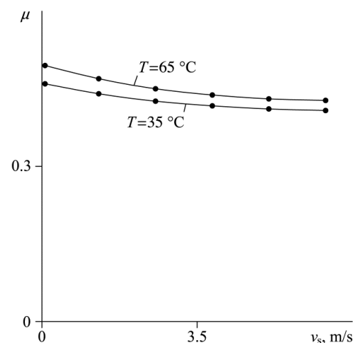
Fig. 2. Friction coefficient \mu decreasing with the sliding velocity v_s at p = 0.2 \text{ MPa}
