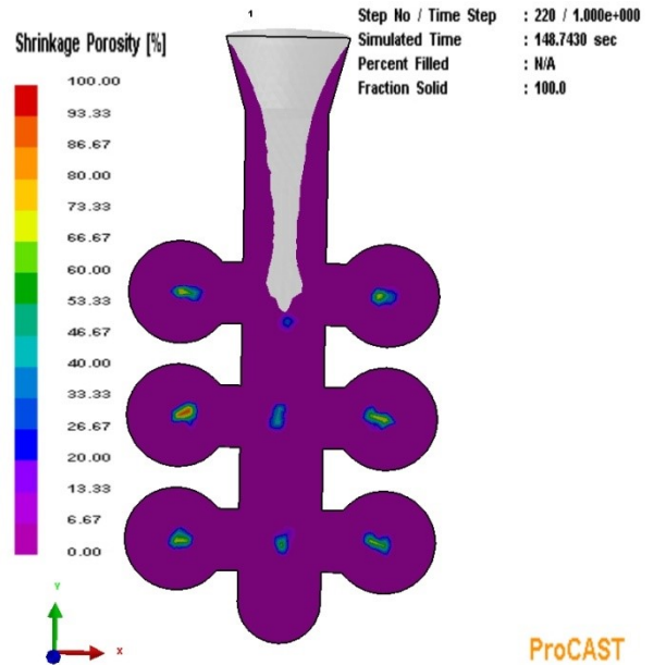
Fig.3. The result of the distribution of shrinkage defects across the section
