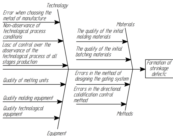
Fig. 5. Diagram of parameters affecting the formation of shrinkage defects
