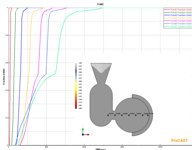
Fig. 8. The dependence of the formation of a solid phase in the body casting time
