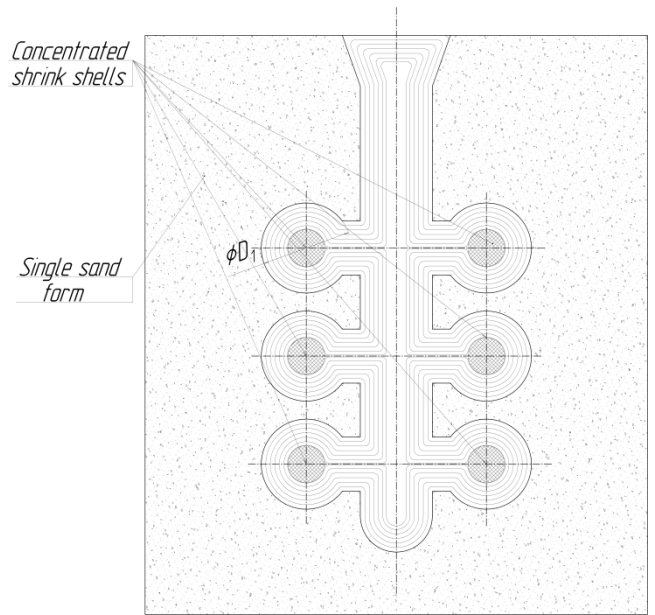
Fig. 2. Isotherms of the process of solidification of the system upon contact of the melt with the form
