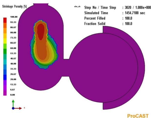
Fig. 9. Porosity distribution in casting over the section
