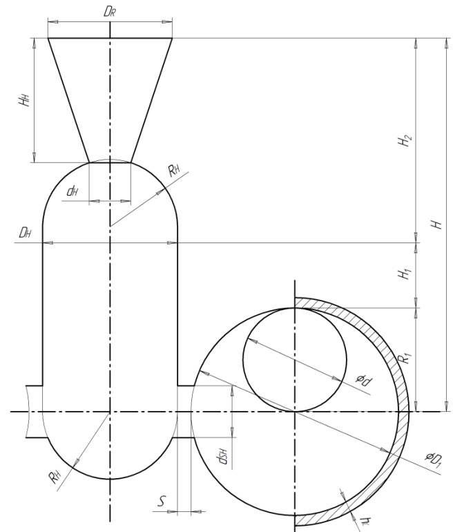
Fig. 6. Sprue and supply system: D_R – upper diameter of the riser; H_H – height of the hood; d_H – bottom diameter of the hood; D_1 – diameter of the ball; D_H – diameter of the head; R_H – radius of the head; d_1 – diameter of the inscribed circle in the thermal node; d_{SH} – diameter of the supply hole; S – supplier length; H_1 – head height, compensating for the shrinkage of the thermal unit of the cast section; H_2 – height of head, compensating for shrinkage of head, compensating, in turn, for shrinkage of the cast section; H – total system height; h_C – thickness of the cooler.
