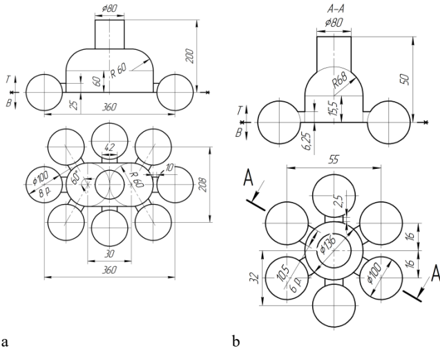
Fig. 1. Diagrams of sprue and supply systems for casting spherical grinding bodies into a sand mold with a horizontal joint
