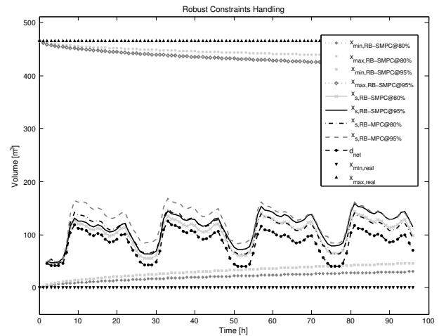
Fig. 3. Risk averse mechanism using the RB-MPC and RB-SMPC approaches.
