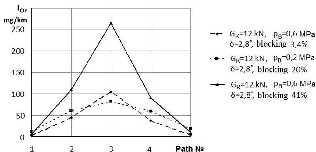
Fig. 9. Relative wearing of the tire on paths at straight motion and \alpha_o = 0^\circ , \delta = 2,8^\circ
