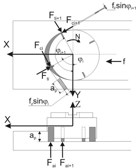
Fig. 1. Geometry of the end milling process
