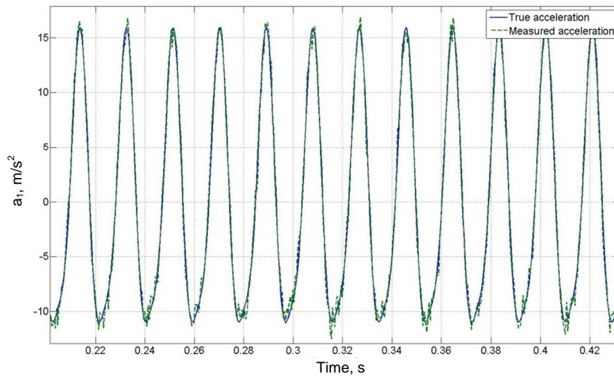
Fig. 5. Sample acceleration signal without and with random error
