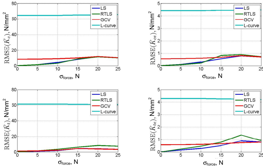
Fig. 7. Influence of force measurements error on the estimation accuracy
