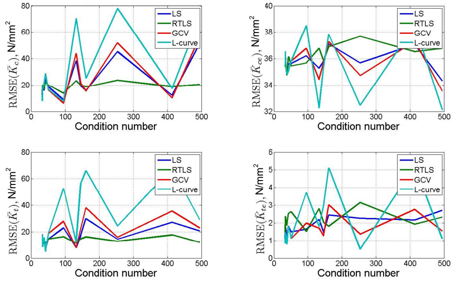
Fig. 8. Influence of the FRF matrix conditioning on the estimation accuracy
