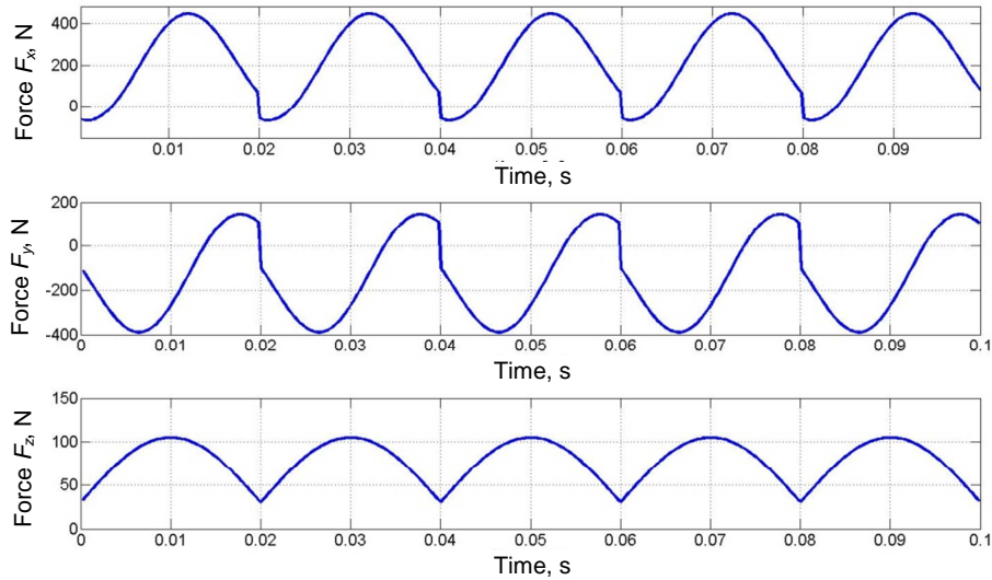
Fig. 4. Cutting forces exciting the investigated structure
