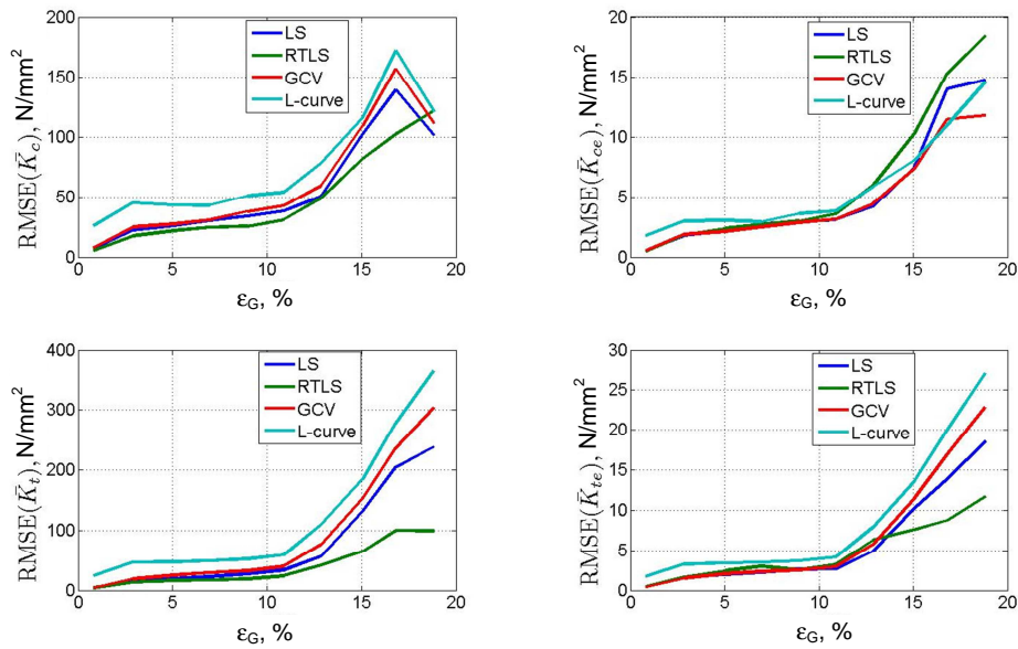
Fig. 9. Influence of the FRF matrix error on the estimation accuracy
