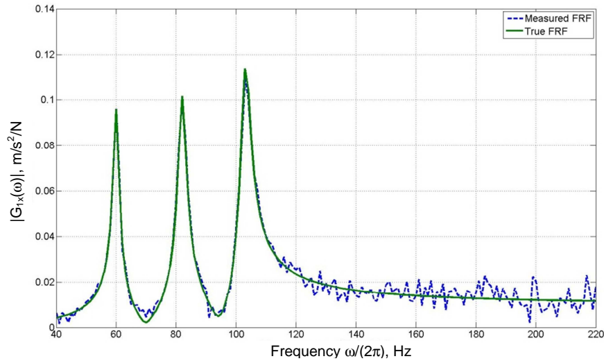
Fig. 3. Amplitude of the “true” and “measured” frequency response function G1x(\omega)
