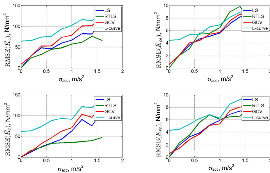
Fig. 6. Influence of acceleration measurements error on the estimation accuracy
