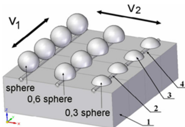
Fig. 6. Solid model of EN-GJS-400/AC-47000 + 10% Al 2 O 3 F contact with fibers parallel ( V_1 ) and perpendicular ( V_2 ) movement to the friction direction: 1 – matrix, 2 – fiber; 3 – grafpite, 4 – transient layer
