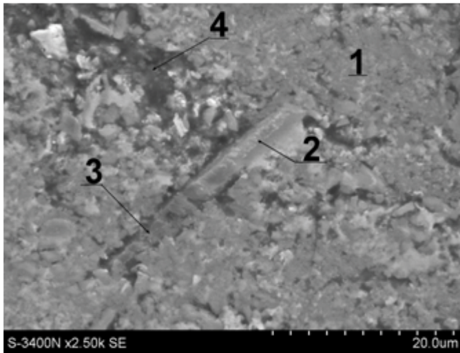
Fig. 12. The fiber of the reinforcing phase in one part broken and in the other protruding from the surface: 1 – matrix, 2 – fiber partially worn, 3 – fiber incrustated in matrix, 4 – valley in matrix action as oil depot
