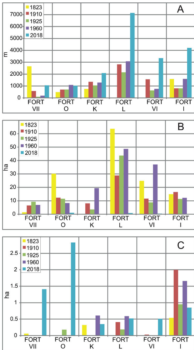
Fig. 4. Changes in selected hydrographic features in the nearest area around the forts of the Terespol Fortification (1823–2018): A – water-course length; B – wetland area; C – area of surface water bodies; source: own study
