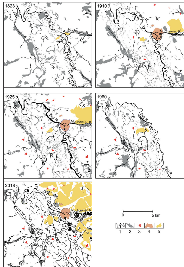
Fig. 2. Location of hydrographic features around the Brest Fortress (1823–2018); 1 = surface waters: rivers, ditches, fluvial lakes (Pol. bużyska), other water bodies; 2 = wetlands; 3 = forts in defensive rings; 4 = Citadel; 5 = urban development; source: own study
