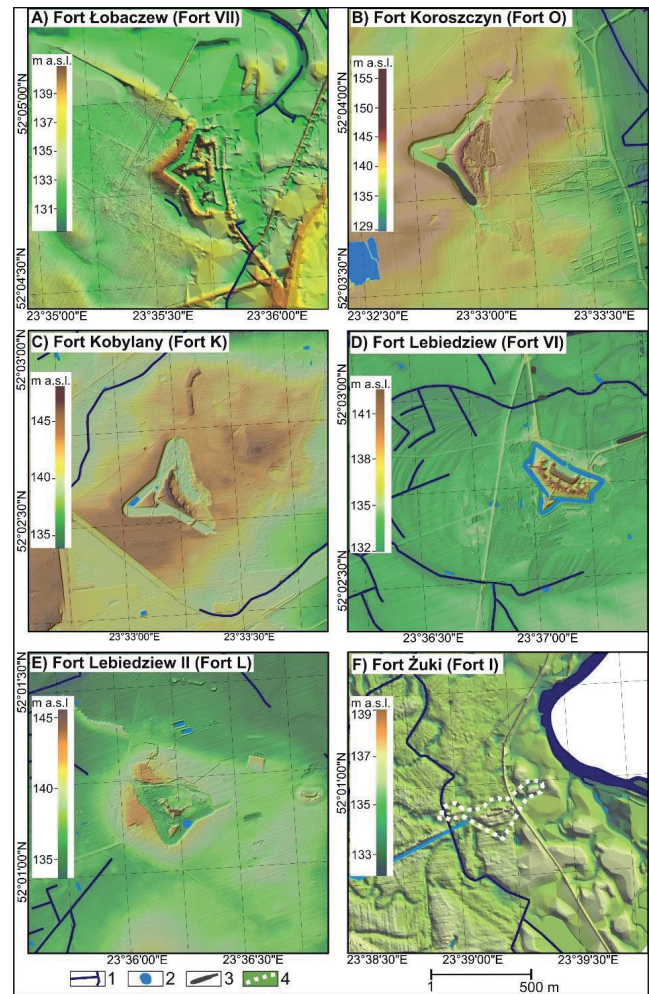
Fig. 3. Transformations of hypsometry area around the forts of the Terespol Fortification (2018); 1 = watercourses; 2 = surface water bodies; 3 = wetlands; 4 = the original range of Fort Żuki; source: own study based on GUGiK [undated]
