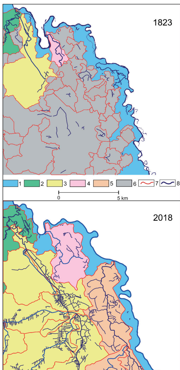
Fig. 6. Changes in the catchment area and watersheds within the Terespol Fortification: 1823 – before the construction of the Brest Fortress; 2018 – at present according to Map of Hydrographic Division of Poland; 1 = direct catchment of Bug; 2 = Dolna Krzna catchment; 3 = Czapelka catchment; 4 = Kosomina catchment; 5 = Doplwy spod Kolonii Dobratycze catchment; 6 = isolated or poorly drained catchments; 7 = topographic watersheds; 8 = watercourses; source: own study
