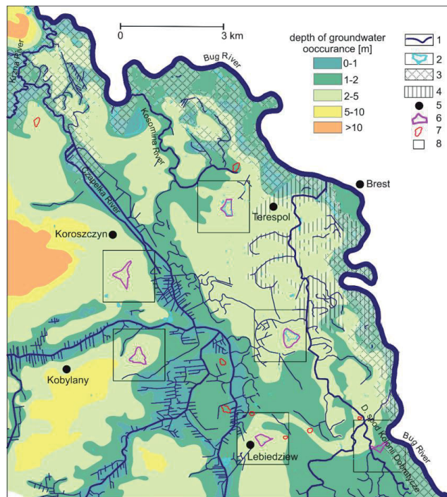
Fig. 5. Contemporary water resources within the Terespol Fortification; 1 = major watercourses and minor drainage ditches; 2 = surface water bodies; 3 = area flooded with water from the Bug river (risk of flood every 10 years); 4 = flood zone acc. to map of 1910; 5 = selected villages; 6 = remains of permanent forts; 7 = remains of field forts; 8 = study plots area (1.5 km × 1.5 km) for individual forts of the Terespol Fortification; Source: own study based on GUGiK undated and PGW Wody Polskie undated
