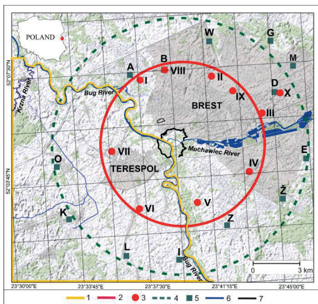
Fig. 1. Major fortifications of Brest Fortress; 1 = area of Terespol Fortification, 2 = 1 st ring of forts, 3 = forts of the 1 st ring, 4 = 2 nd ring of forts, 5 = forts of the 2 nd ring, 6 = major surface water bodies, 7 = Brest Fortress; source: own elaboration
