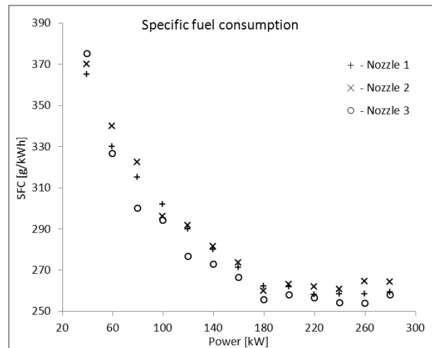
Fig. 3. Specific fuel consumption
