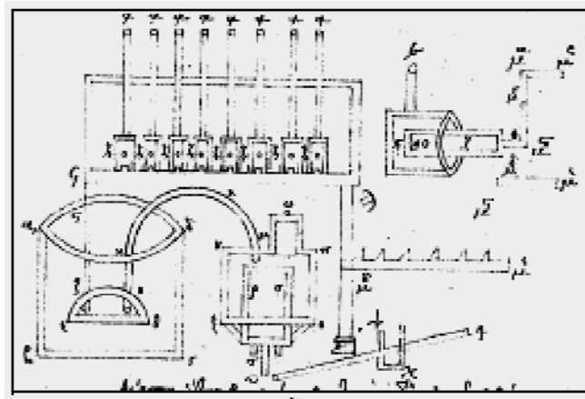
Fig.9. A hydraulic organ designed in the 2-nd century B.C. by Heron of Alexandria as redrawn in 15th century.
