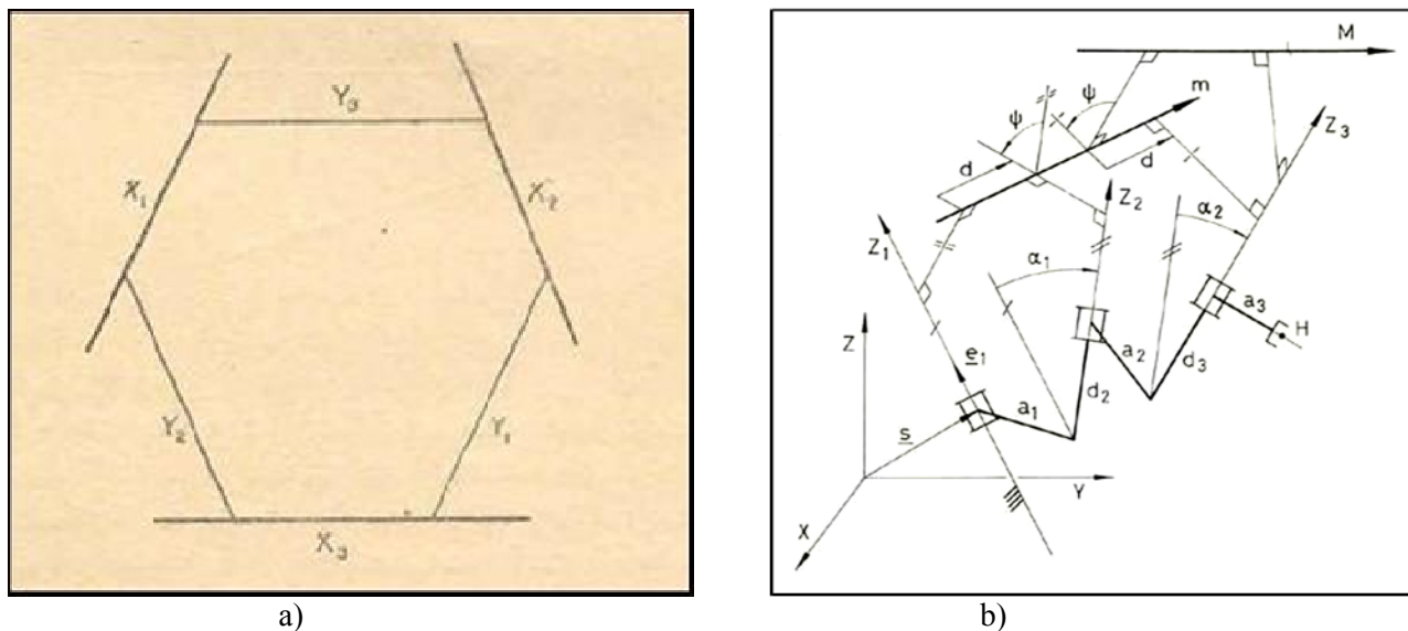
Fig.3. A scheme for Screw Triangle of a 3R manipulator: a) by Bricard in 1926,) b) as drawn today.
