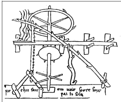
Fig.8. An automatic wood sawing machine by Villard de Honnecourt in the 13-th century.
