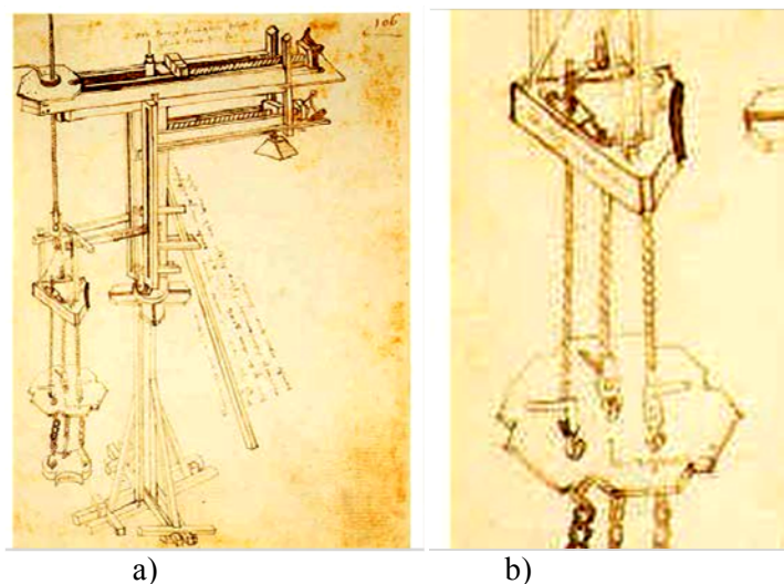
Fig.4. An early cable parallel manipulator in crane by Filippo Brunelleschi in 1420: a) the crane system; b) zoomed view of an early cable-driven parallel manipulator.
