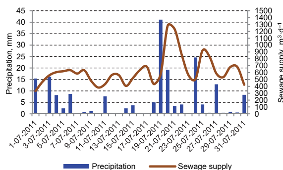
Fig. 2. Effect of precipitation on the increase of sewage amount entering the treatment plant in July 2011; source: own study
