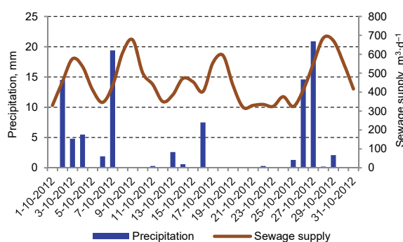
Fig. 3. Effect of precipitation on the increase of sewage amount entering the treatment plant in October 2012; source: own study
