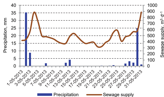
Fig. 4. Effect of precipitation on the increase of sewage amount entering the treatment plant in May 2013; source: own study
