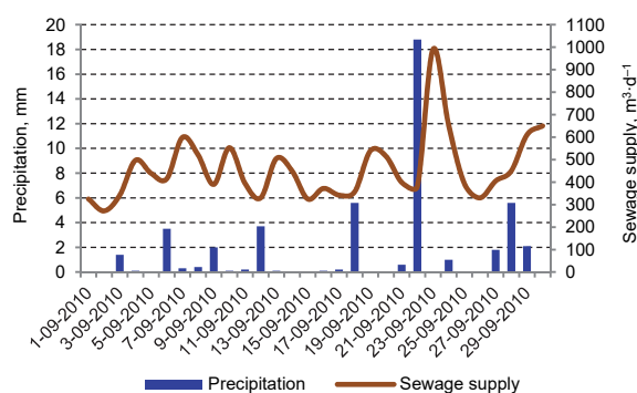
Fig. 1. Effect of precipitation on the increase of sewage amount entering the treatment plant in September 2010; source: own study
