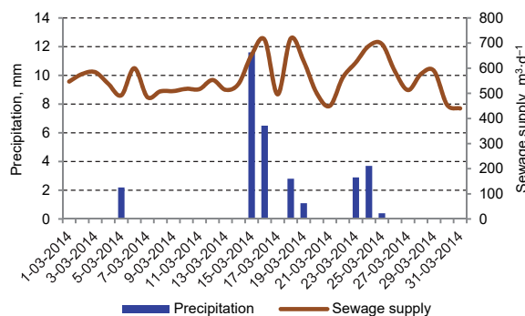
Fig. 5. Effect of precipitation on the increase of sewage amount entering the treatment plant in March 2014; source: own study
