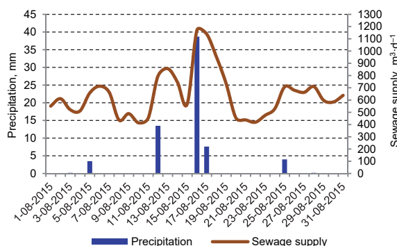
Fig. 6. Effect of precipitation on the increase of sewage amount entering the treatment plant in August 2015; source: own study
