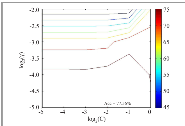
Fig. 1. A 10-fold cross validation done using LIBSVM. (See color pictures online at www.nit.eu/publications/journal-jtit )
