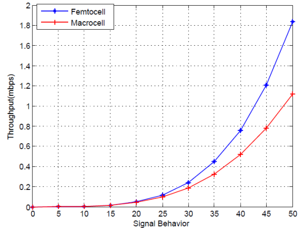
Fig 6: Signal behavior of femtocell over macrocells in an indoor environment
