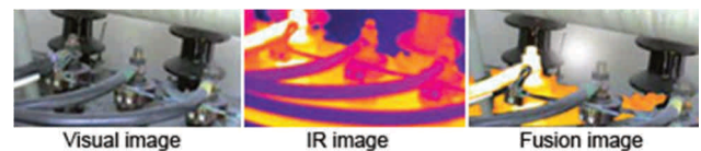
Fig. 2. Comparing images (from left side) in visible light, in infrared and using fusion technology [1]
