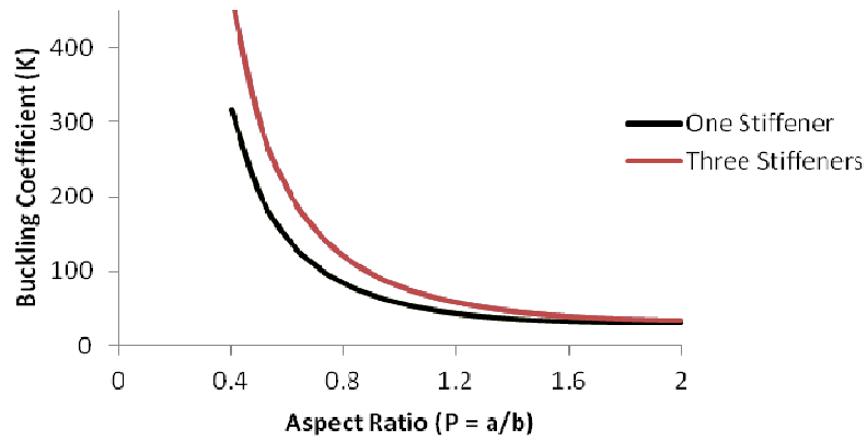
Fig.6. Buckling coefficient vs aspect ratio for CCCC stiffened plate for \gamma=5, \delta=0.05 .
