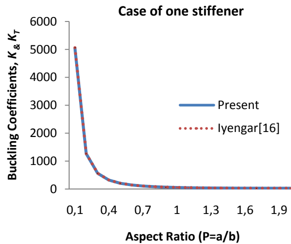
Fig.2. Buckling coefficients vs aspect ratio for CCCC stiffened plate for \gamma = 5, \delta = 0.05 .
