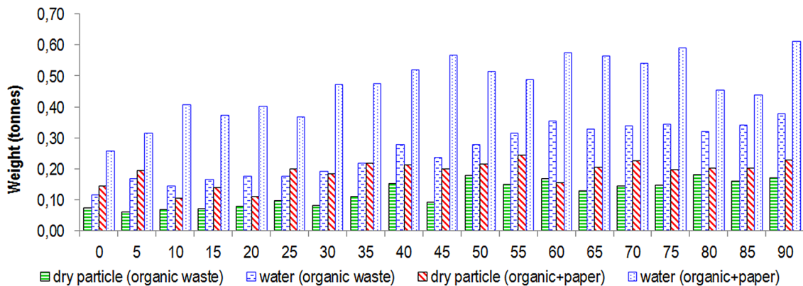
Figure 4. Simulation of solid weight and water weight in 1 m 3 of MSW pile, according to the density data and moisture content of the MSW from the test results
