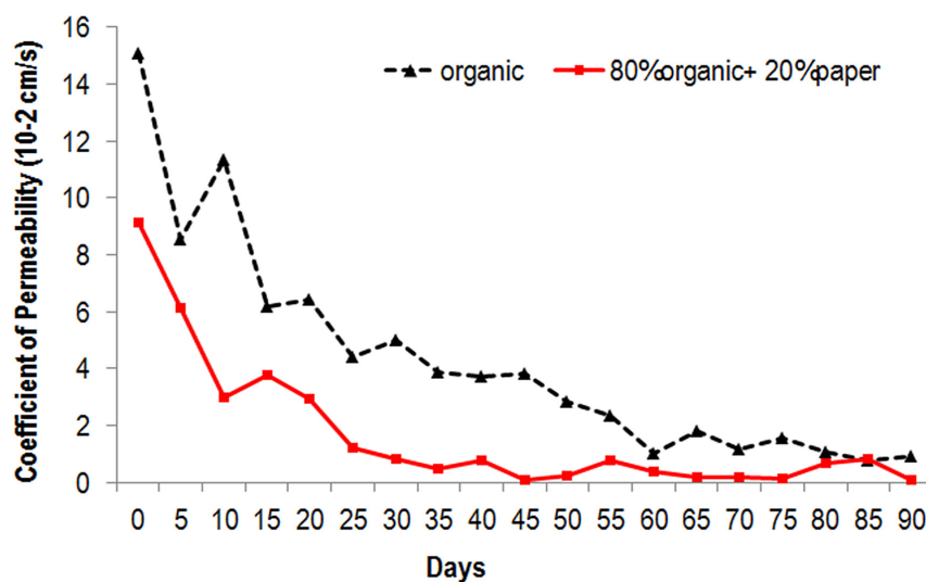
Figure 5. Permeability coefficient of MSW sample
