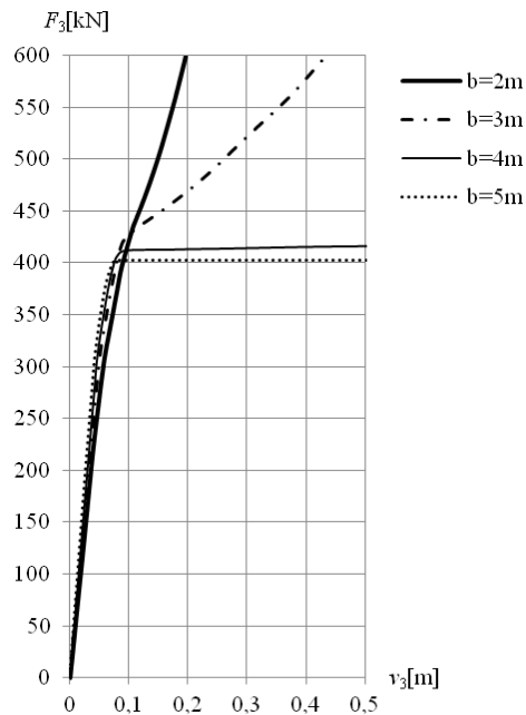
Fig. 3. Load F_3 versus displacement v_3 diagram for system ( F_5>0 )
