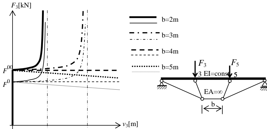
Fig. 5. Load F_3 versus displacement v_3 diagram for systems with dead load ( F_5 > 0 ) – more thickness lines and without dead load ( F_5 = 0 ) – thin lines
