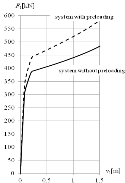
Fig. 8. Load F_1 versus displacement v_1 diagram for the viaduct
