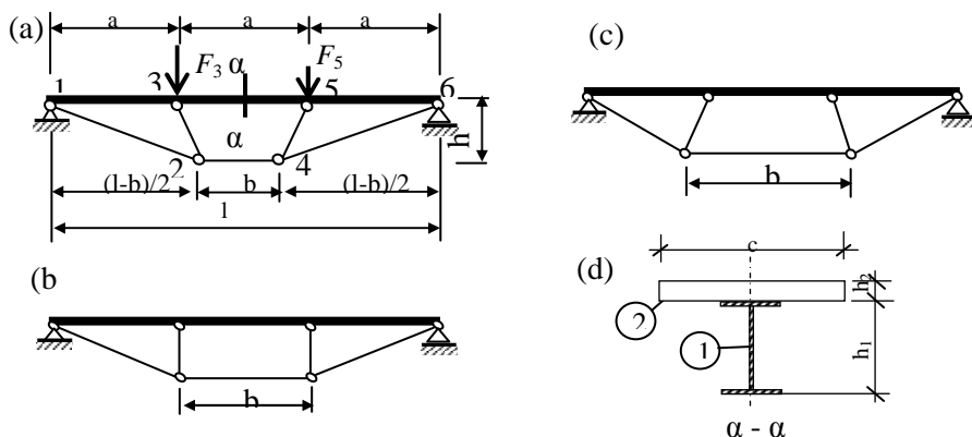
Fig. 1. Scheme with loading of the rod system: (a) b < l/3 ; (b) b = l/3 ; (c) b > l/3
