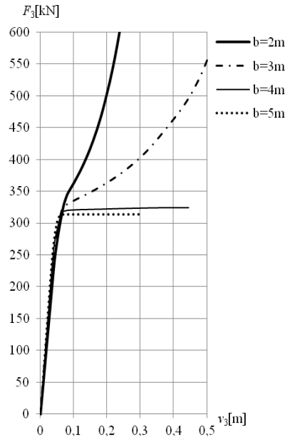
Fig. 2. Load F_3 versus displacement v_3 diagram for system without preloading ( F_5=0 )
