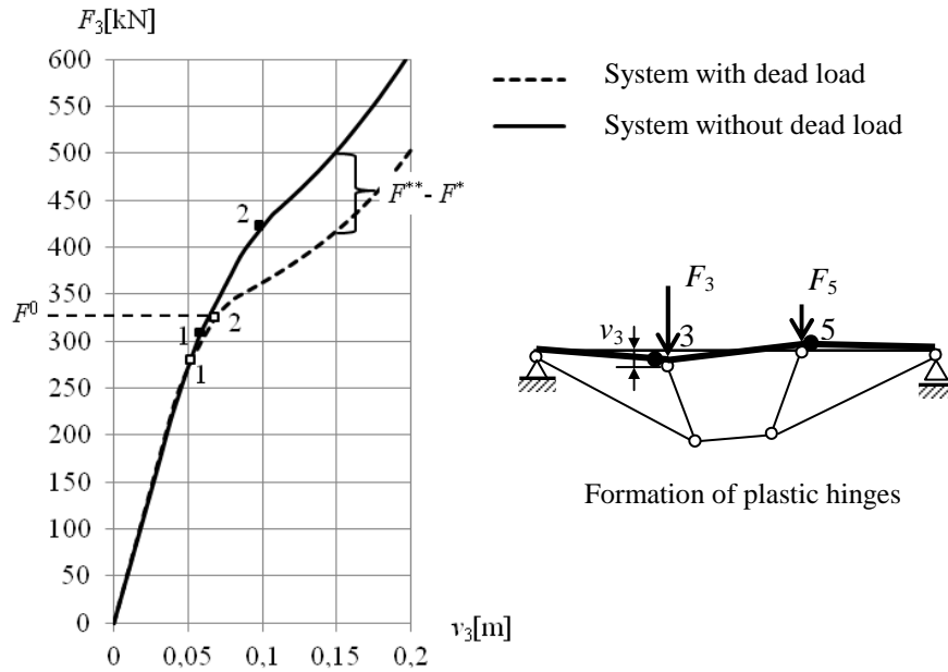
Fig. 4. Load F_3 versus displacement v_3 diagram for b = 2 m
