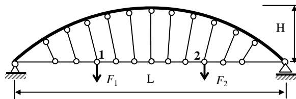
Fig. 7. Simplified scheme and loading of the viaduct WD-22
