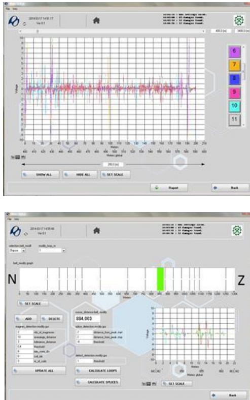
Fig. 5. RAW data analysis and loop and splice detection windows
