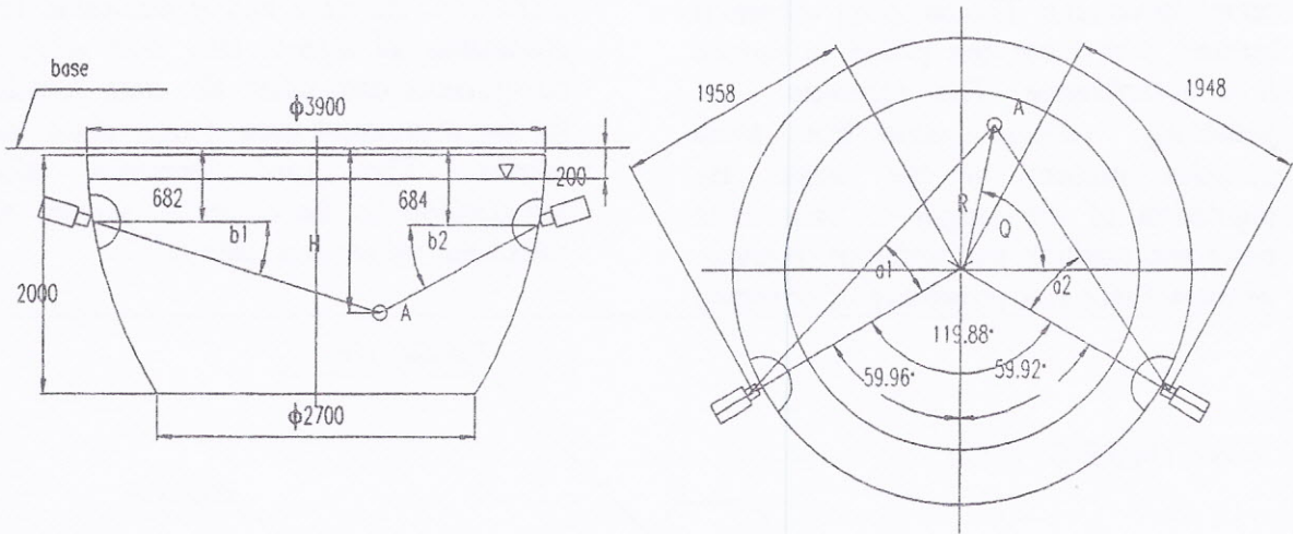
Fig.2. The geometry of measurement system
