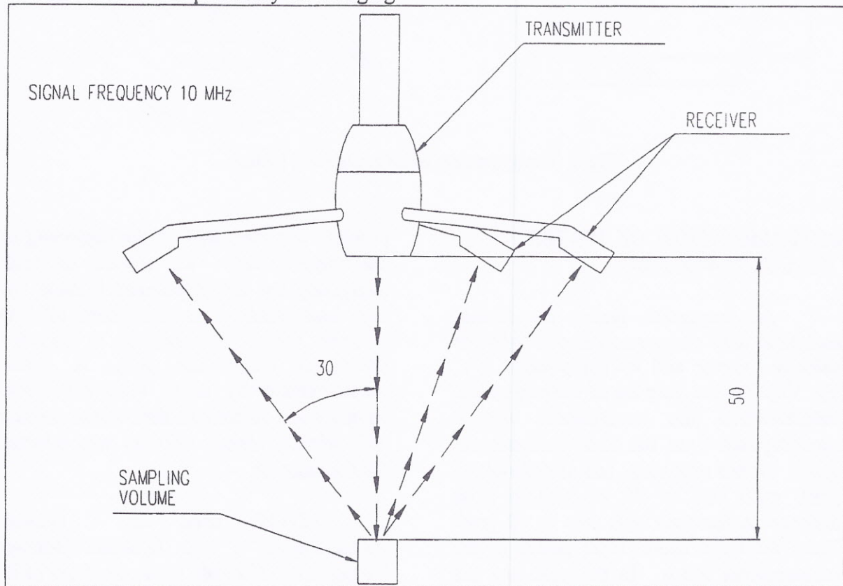
Fig.3. Principle of operation of ADV
