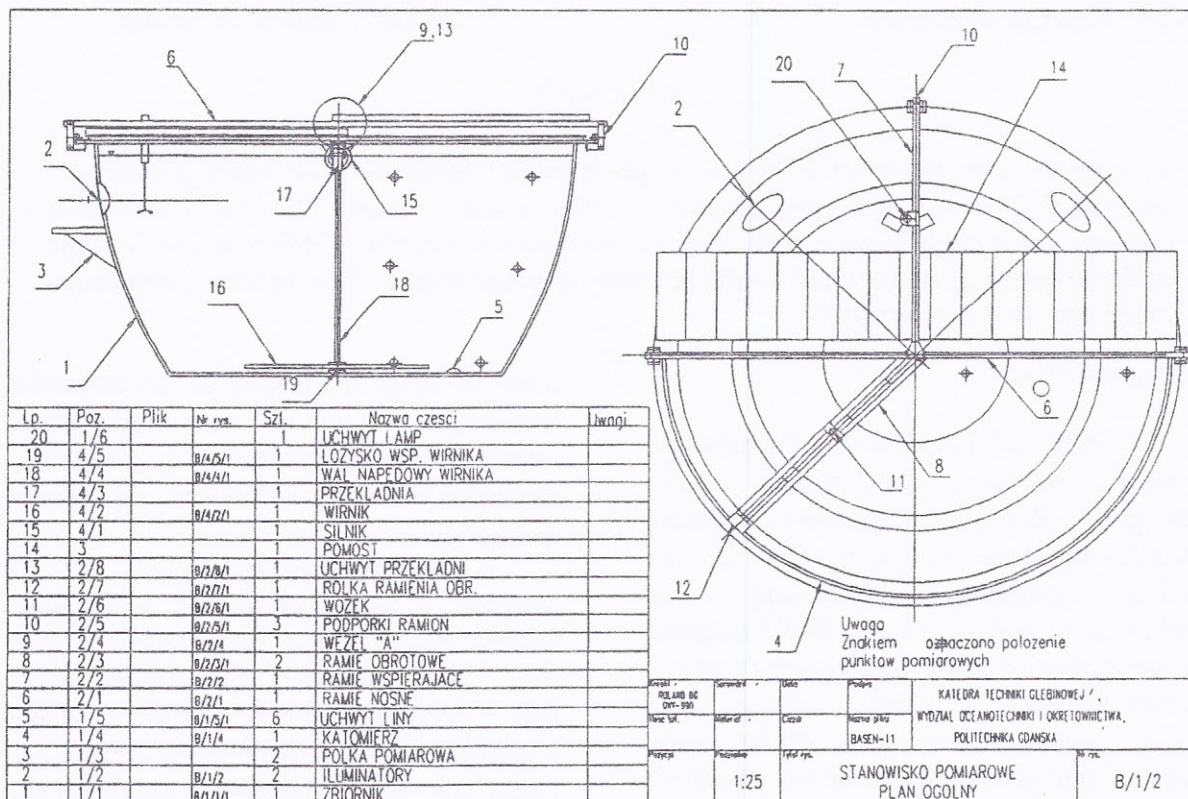
Fig.1. The test stand
