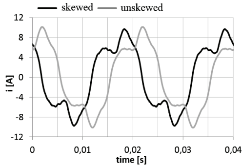
Fig. 9. Currents in time domain for the skewed and unskewed motor stator (rated load)
