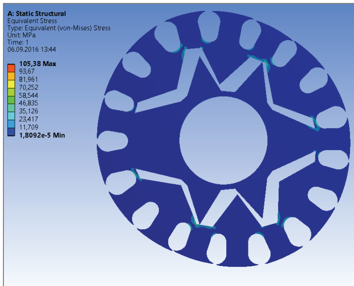
Fig. 3. Mechanical analyses of rotor sheet under stress: n_{\text{rotor}} = 1.2n_s , T_{\text{load}} = 20 T_n
