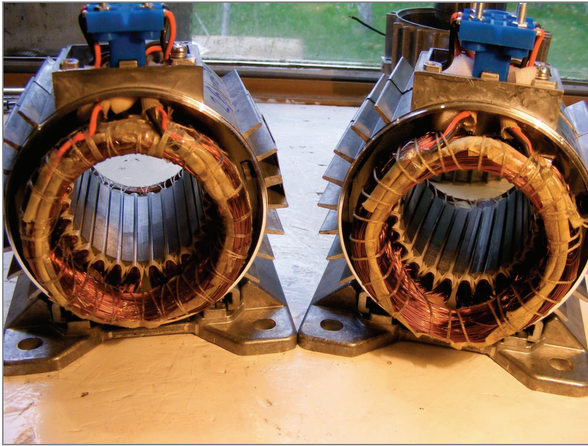
Fig. 5. Stators of the built motors: unskewed (left) and skewed (right)
