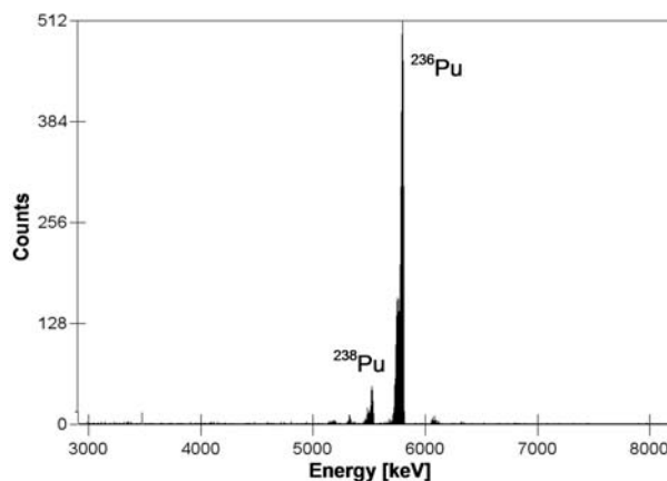
Fig. 3. Alpha spectra of a urine sample with ^{238}\text{Pu} activity above MDA.
