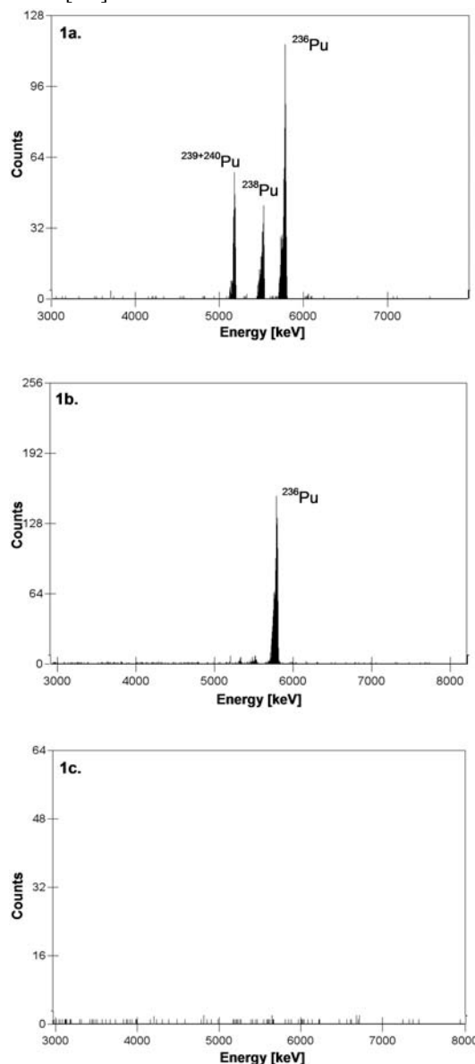
Fig. 1. Alpha spectra of a) urine sample with plutonium isotopes ( 236 Pu, 238 Pu, 239+240 Pu), b) urine sample with tracer ( 236 Pu), c) blank sample.
