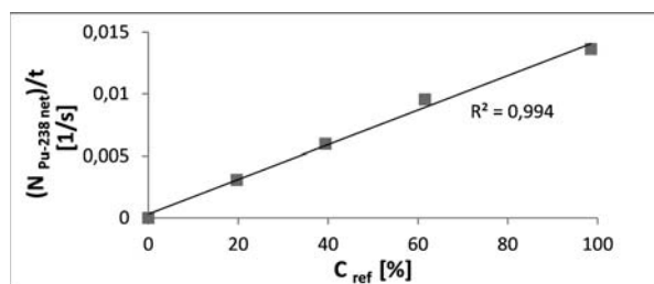
Fig. 2. Assessment of linearity of the determination method of plutonium activity.
