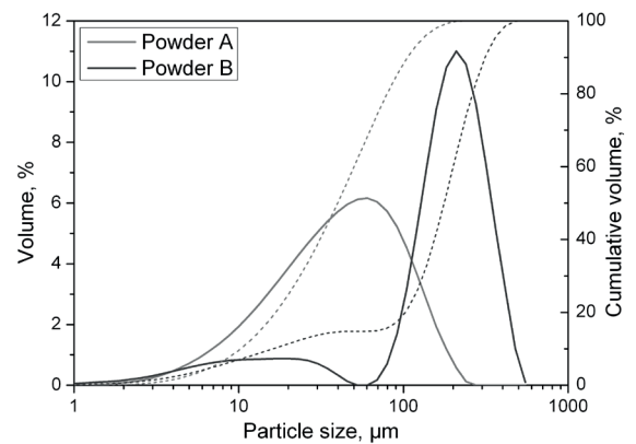
Fig. 2. Particle-size distribution of the Tb_{0.3}Dy_{0.7}Fe_{1.9} powders used in the experiments
