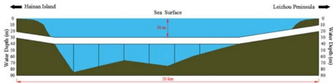
Fig. 4. Longitudinal profile of proposed SFT on central line
