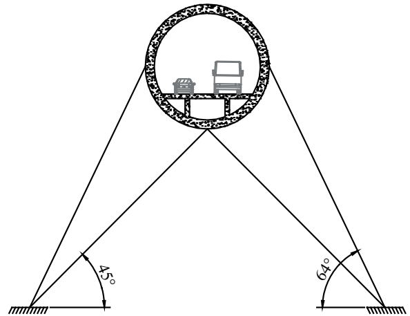
Fig. 6. Proposed inclined configuration of cables
