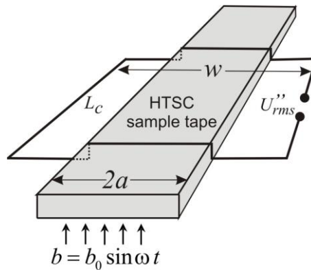
Fig. 8. Arrangement of the sample tape with a saddle pick-up coil. The external magnetic field b is oriented perpendicularly to the plane of the sample of the width 2a . The pick-up sensing coil of the width w and the length L_c is wrapped around the tape. The loss voltage U''_{rms} is measured by the lock-in amplifier in phase with the external magnetic field b .
