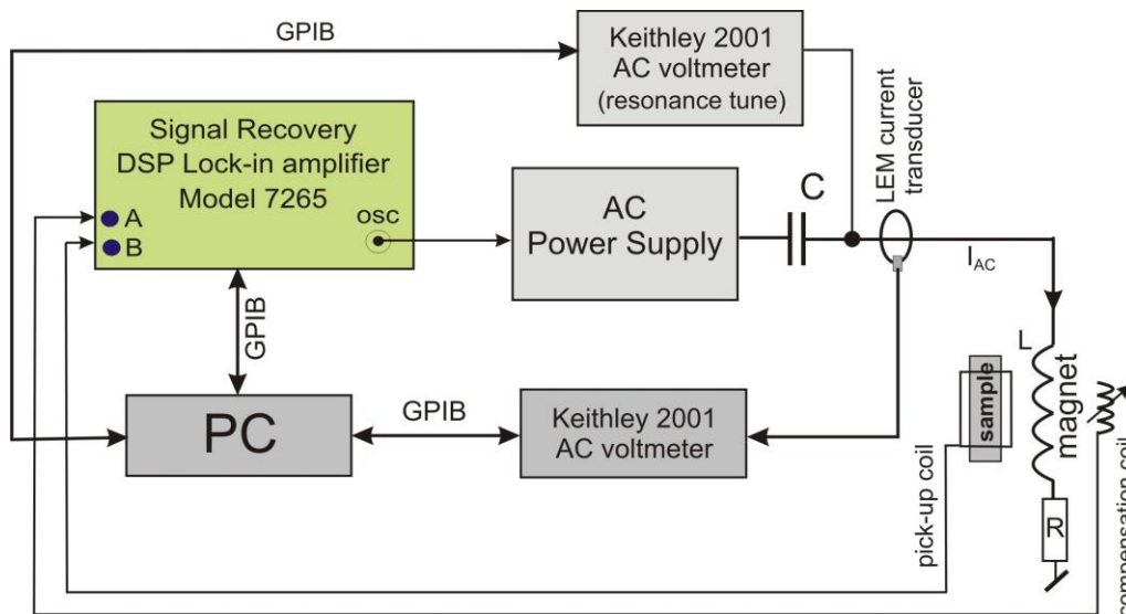
Fig. 7. Block diagram of the AC magnetization losses measurement system. For details see text and Fig. 8.
