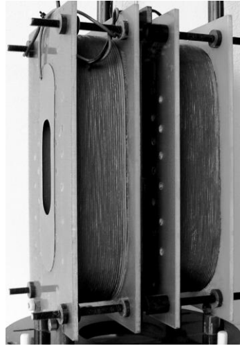
Fig. 5. Home-made race-track coils system.
