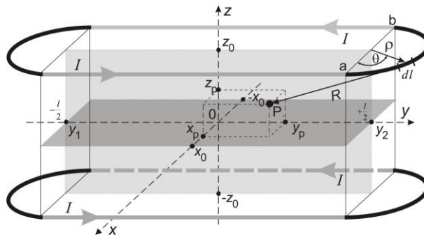
Fig. 3. Schematic view of the race track-coil wire turns for calculations of the magnetic field distribution originating from the semicircular ends of the coil turn.
