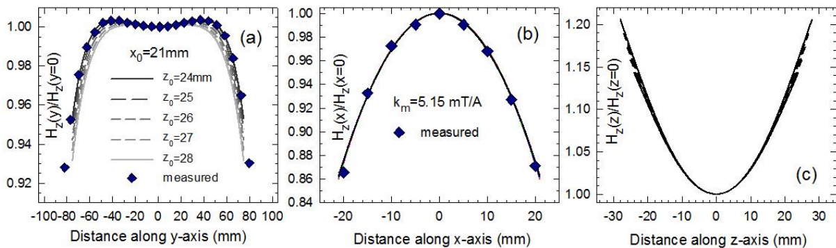
Fig. 6. Calculated (lines) and determined experimentally (points) H_z -magnetic field component distributions along three main axes X, Y, Z, as a function of the coils separation distance z_0 . The magnetic field values are normalized to the value of the field in the geometrical center of the coils assembly.
