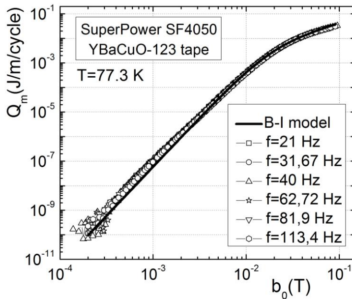
Fig. 9. AC magnetization losses Q_m versus magnetic field amplitude b_0 , for different frequencies (21 to 113.4 Hz). The solid line (B-I) is according to the Brandt-Indenbom theoretical model [14].
