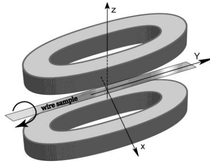
Fig. 1. General view of the Helmholtz race-track coil assembly.
