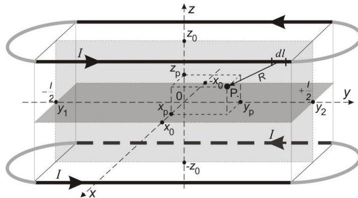
Fig. 2. Schematic view of the race track-coils turns for calculations of the magnetic field originating from the straight line elements. For clarity, only two single wire turns forming the Helmholtz coils system are shown. For parameters see text.
