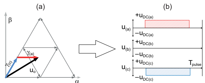
Fig. 5. a) the duty cycles in modulation strategy I; b) corresponding phase voltage waveforms
