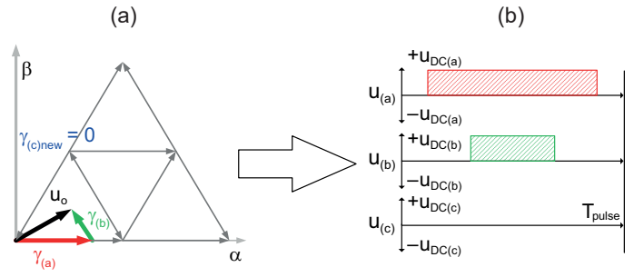
Fig. 9. The duty cycles in modulation strategy III (a) and corresponding phase voltage waveforms (b) in the case of zero duty cycle for H-bridge in phase “c”
