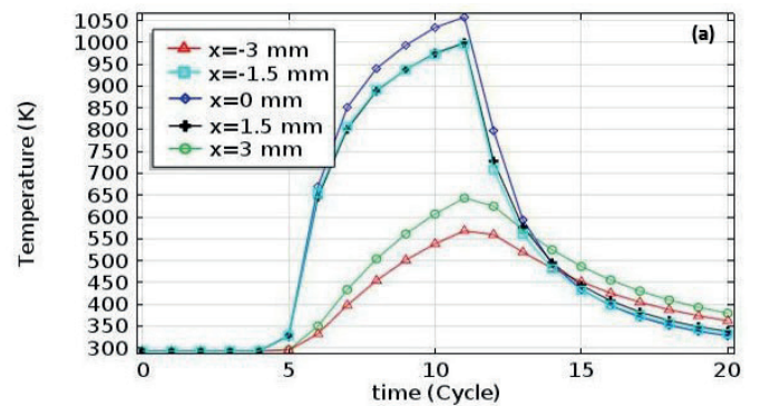
Fig. 12. Predicted cooling and heating rates at center and around the single spot weld for 25.3 kA welding current and 6 cycles welding time
