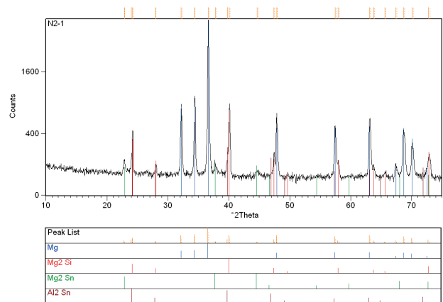
Fig. 3. X-ray diffraction pattern of Mg-5Si-7Sn-2Al alloy
