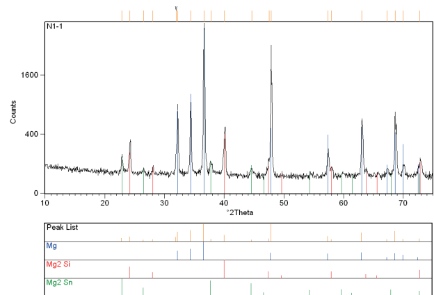
Fig. 2. X-ray diffraction pattern of Mg-5Si-7Sn alloy
