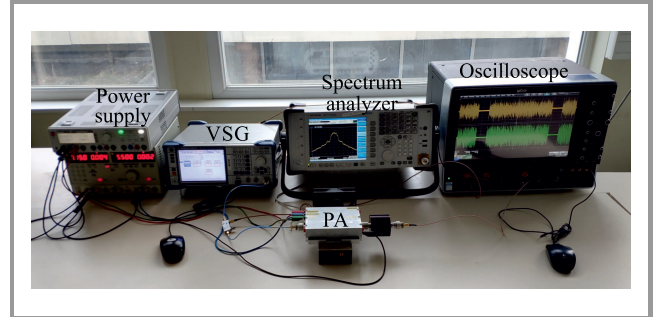
Fig. 5. Experimental setup.
