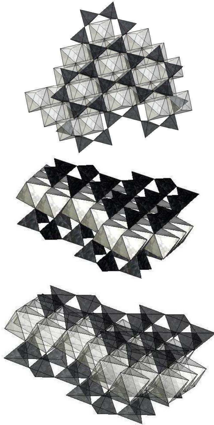
Fig. 12. Geometry of the three sub-layers joined together
