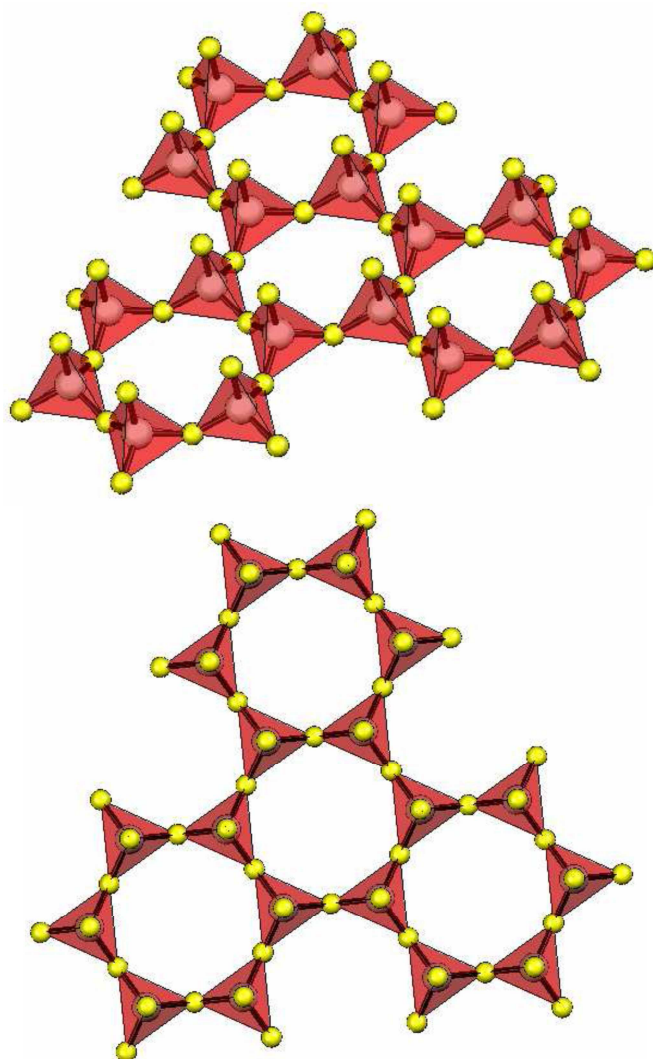
Fig. 11. Atomic structure of the outer tetrahedral sub-layer
