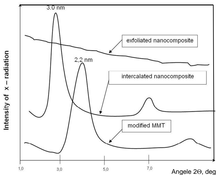
Fig. 19. Diffraction pattern obtained from SAXS method
