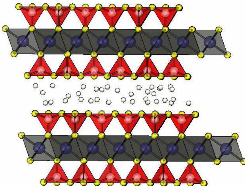
Fig. 14. Side view of the MMT packet with the visible gallery filled with cations
