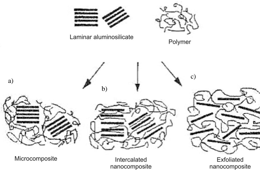
Fig. 16. Schematic structures of MMT-polymer nanocomposite [3, 11]: a) mikrokomposite, b) intercalated nanocomposite, c) exfoliated nanocomposite
