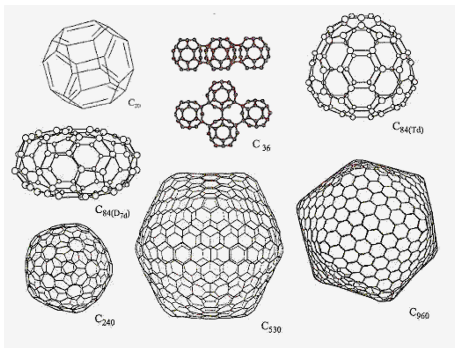
Fig. 2. Some examples of common and giant fullerenes [6]
