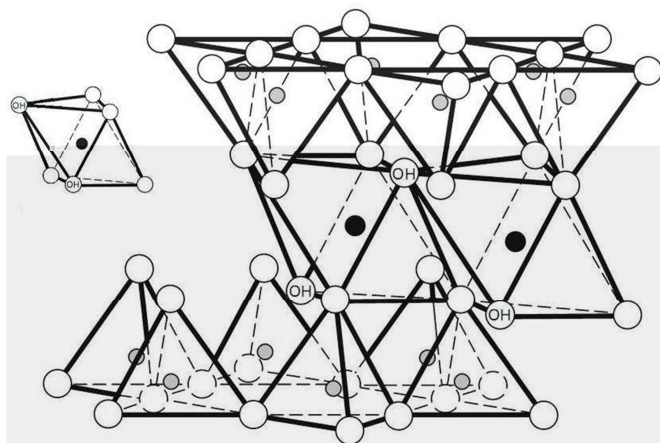
Fig. 7. Fragment of MMT structure with the visible hydroxide group [9]
