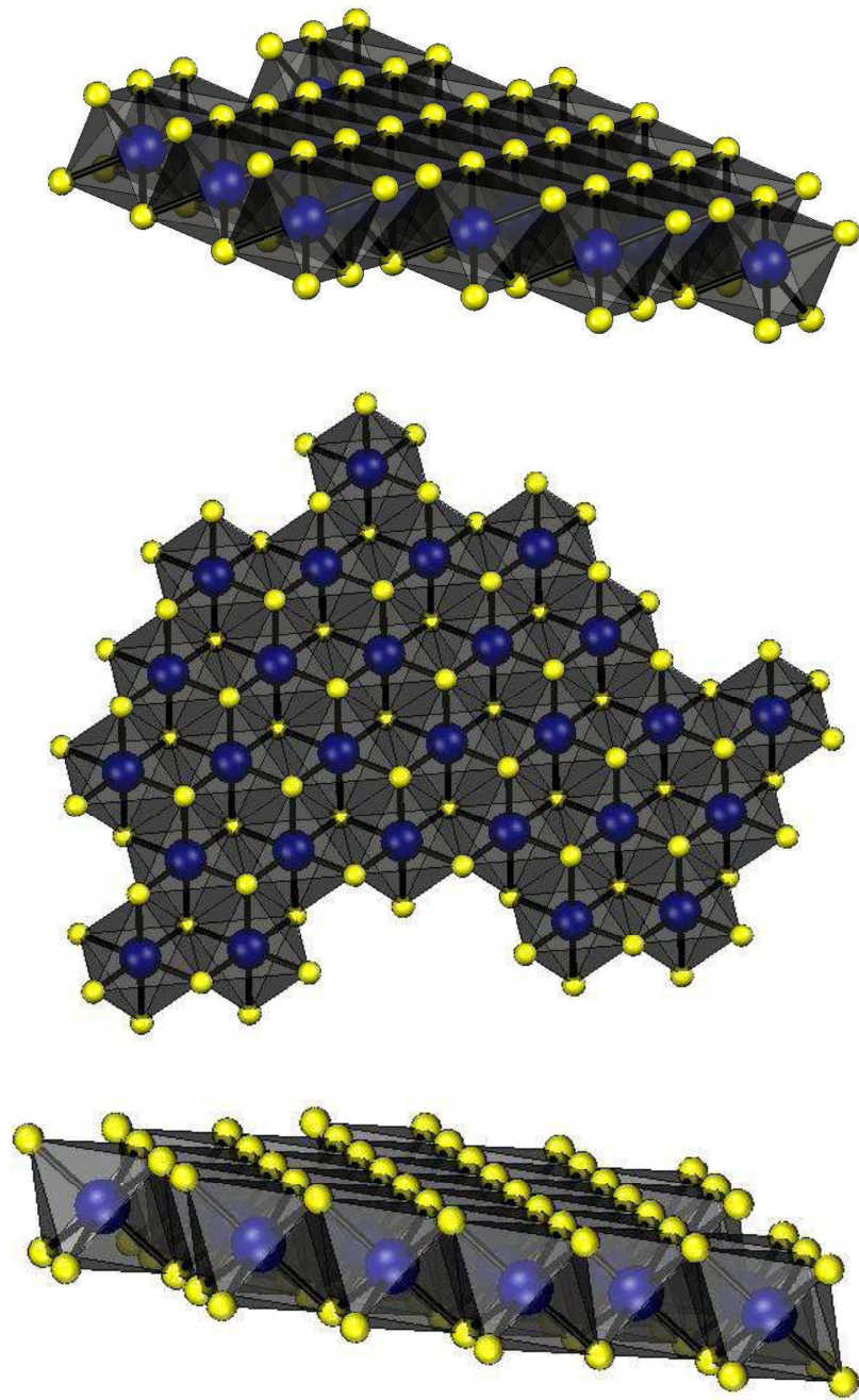
Fig. 9. Atomic structure of the inner, octahedral sub-layer
