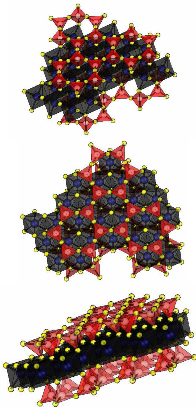
Fig. 13. Atomic structure of the complete MMT layer
