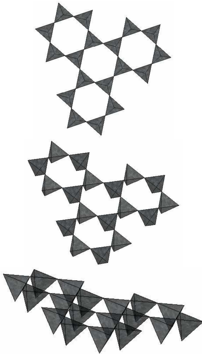
Fig. 10. Geometry of the outer, tetrahedral sub-layer
