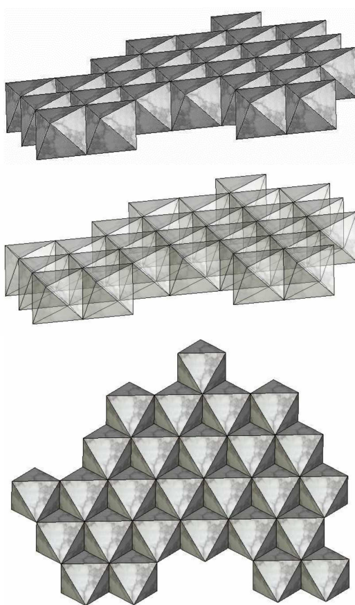
Fig. 8. Geometry of the inner, octahedral sub-layer
