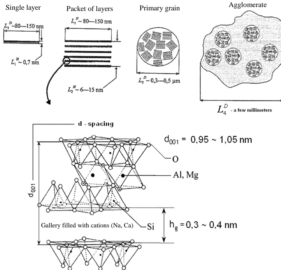
Fig. 15. Complete structure of the MMT agglomerate [11, 12]
