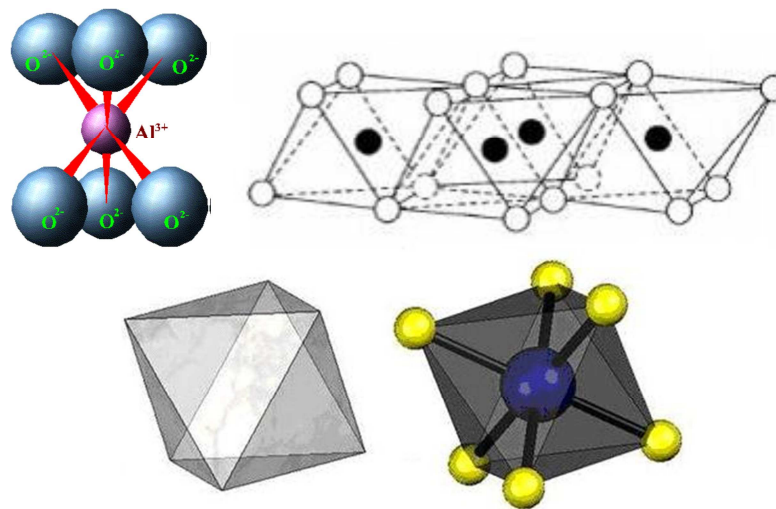
Fig. 6. Regular octahedrons set up by aluminum atoms (middle) and oxygen atoms (corners)
