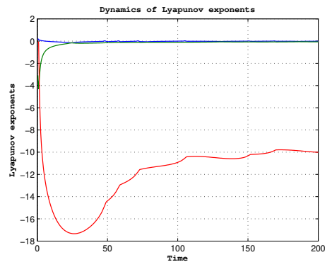
f) Lyapunov exponents L_1 = -0.011976 , L_2 = -0.0065696 , L_3 = -10.010001 of (19) with parameters given in (20) and I = 3.25 , r = 0.0145
