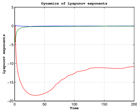
a) Lyapunov exponents L_1 = -0.002382 , L_2 = -0.059071 , L_3 = -10.738918 of (19) with parameters given in (20) and I = 3.25 , r = 0.008
