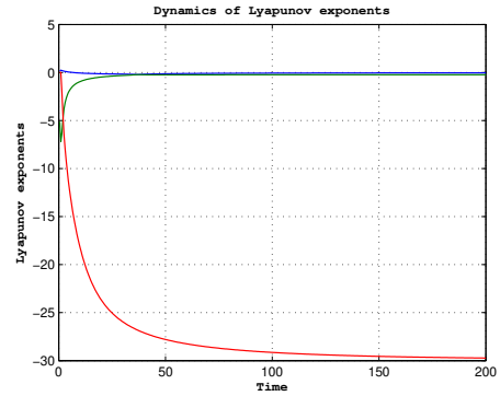
d) Lyapunov exponents L_1 = -0.032696 , L_2 = -0.226844 , L_3 = -29.730009 of (19) with parameters given in (20) and I = 3.25 , r = 0.0001
