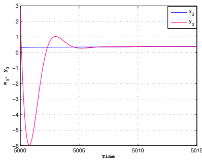
c) synchronization of intrinsic current (the exchange of ions through slow ionic channels) when the injected current in the neuron I = 1 and the ratio of time scales between spiking (fast dynamics) and resting (slow dynamics) r = 0.001
