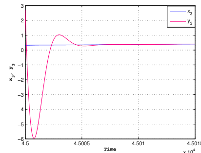
f) synchronization of the exchange of ions through slow ionic channels when the injected current in the neuron I = 1.5 and the ratio of time scales between spiking and resting r = 0.001
