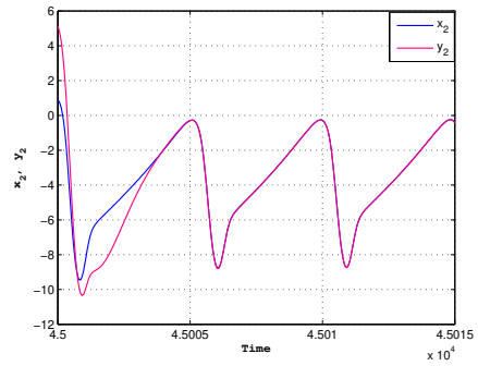
b) synchronization of the exchange of ions across the neuron membrane through fast ionic channels when the injected current in the neuron I = 2 and the ratio of time scales between spiking and resting r = 0.001
