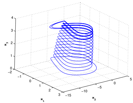
f) (x, y, z) phase portraits of the system (19) with parameters given in (20) and with I = 3.25 for r = 0.01
