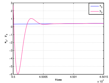
f) synchronization of the exchange of ions through slow ionic channels when the injected current in the neuron I = 3 and the ratio of time scales between spiking and resting r = 0.001
