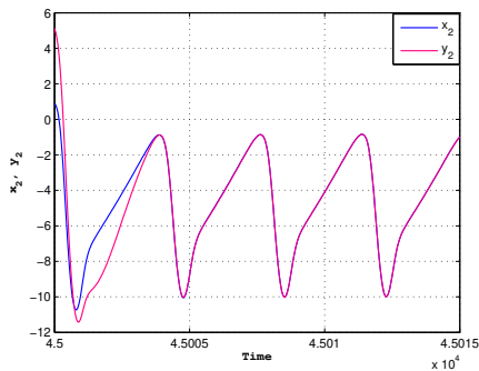
e) synchronization of the exchange of ions across the neuron membrane through fast ionic channels when the injected current in the neuron I = 3 and the ratio of time scales between spiking and resting r = 0.001
