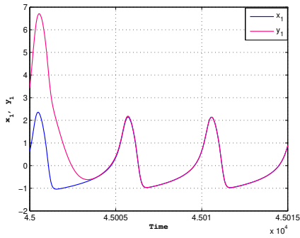
a) synchronization of membrane potential when the injected current in the neuron I = 2 and the ratio of time scales between spiking and resting r = 0.001
