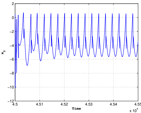
e) Time series portraits of the system (19) with parameters given in (20) and with I = 3.25 for r = 0.05 , a period doubling cascade is observed
