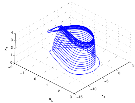
d) (x, y, z) phase portraits of the system (19) with parameters given in (20) and with I = 3.25 for r = 0.0095
