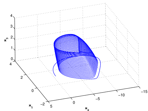
d) (x, y, z) phase portraits of the system (19) with parameters given in (20) with I = 3.25 for r = 0.001
