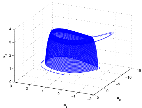
d) (x, y, z) phase portraits of the system (19) with parameters given in (20) and with I = 3.25 for r = 0.002
