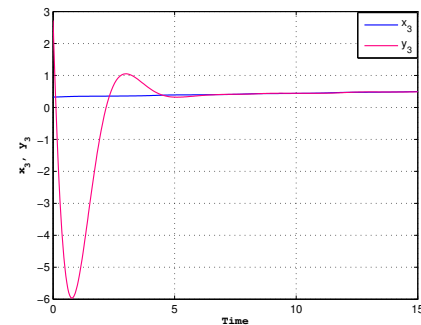
f) synchronization of the exchange of ions through slow ionic channels when the injected current in the neuron I = 3.25 and the ratio of time scales between spiking and resting r = 0.0017
