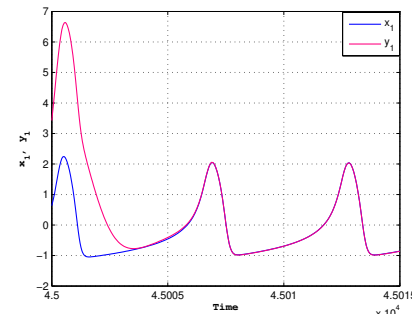
d) synchronization of membrane potential when the injected current in the neuron I = 1.5 and the ratio of time scales between spiking and resting r = 0.001
