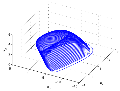
b) (x, y, z) phase portraits of the system (19) with parameters given in (20) with I = 3 for r = 0.001
