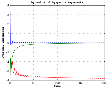
a) Lyapunov exponents L_1 = -0.001829 , L_2 = -0.042157 , L_3 = -3.815855 of (19) with parameters given in (20) and I = 3.25 , r = 0.00041
