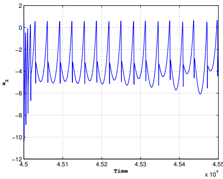
c) Time series portraits of the system (19) with parameters given in (20) and with I = 3.25 for r = 0.03 , a period doubling cascade is observed
