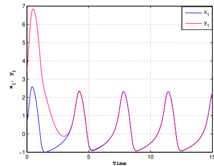
d) synchronization of membrane potential when the injected current in the neuron I = 3.25 and the ratio of time scales between spiking and resting r = 0.0017
