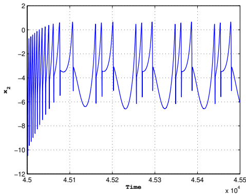
a) Time series portraits of the system (19) with parameters given in (20) and with I = 3.25 for r = 0.011 , a period doubling cascade with a period three solution is observed
