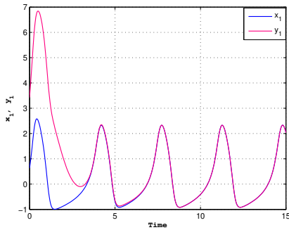
a) synchronization of membrane potential when the injected current in the neuron I = 3.25 and the ratio of time scales between spiking and resting r = 0.0001
