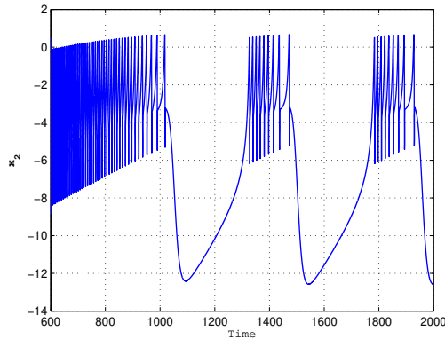
c) Time series portraits of the system (19) with parameters given in (20) with I = 2 for r = 0.001 , the neuron behaviour changes from tonic spiking to bursting is observed
