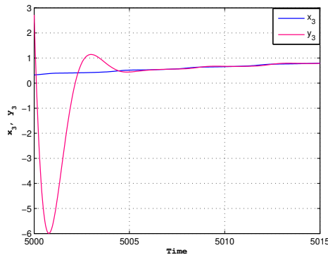
c) synchronization of the exchange of ions through slow ionic channels when the injected current in the neuron I = 3.25 and the ratio of time scales between spiking and resting r = 0.001
