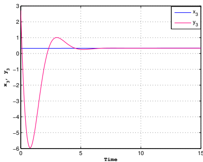
c) synchronization of the exchange of ions through slow ionic channels when the injected current in the neuron I = 3.25 and the ratio of time scales between spiking and resting r = 0.0001
