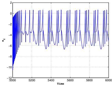
c) Time series portraits of the system (19) with parameters given in (20) and with I = 3.25 for r = 0.0095 , a period doubling cascade with a period three solution is observed
