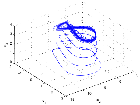
b) (x, y, z) phase portraits of the system (19) with parameters given in (20) and with I = 3.25 for r = 0.03
