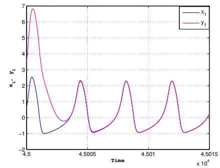
d) synchronization of membrane potential when the injected current in the neuron I = 3 and the ratio of time scales between spiking and resting r = 0.001
