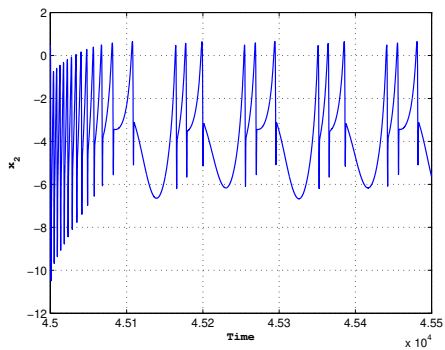
e) Time series portraits of the system (19) with parameters given in (20) and with I = 3.25 for r = 0.01 , a period doubling cascade with a period three solution is observed
