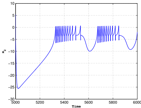
c) Time series portraits of the system (19) with parameters given in (20) and with I = 3.25 for r = 0.002 , the neuron behavior changes from tonic spiking to bursting is observed
