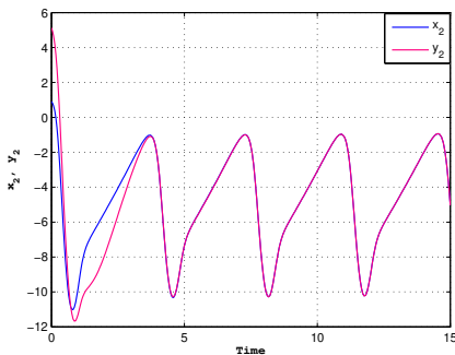
e) synchronization of the exchange of ions across the neuron membrane through fast ionic channels when the injected current in the neuron I = 3.25 and the ratio of time scales between spiking and resting r = 0.0017
