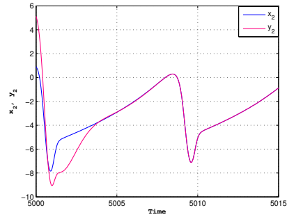
b) synchronization of electrode (the exchange of ions across the neuron membrane through fast ionic channels) when the injected current in the neuron I = 1 and the ratio of time scales between spiking (fast dynamics) and resting (slow dynamics) r = 0.001
