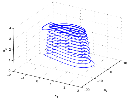
b) (x, y, z) phase portraits of the system (19) with parameters given in (20) and with I = 3.25 for r = 0.011
