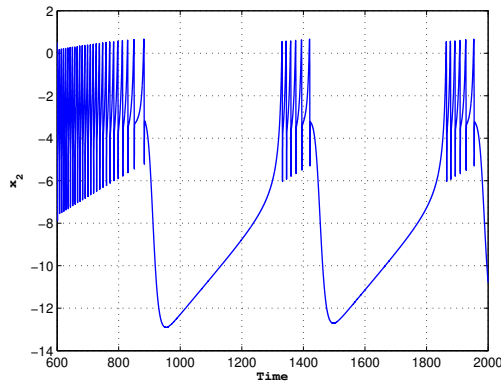
a) Time series portraits of the system (19) with parameters given in (20) with I = 1.5 for r = 0.001 , a period doubling cascade with a period three solution is observed
