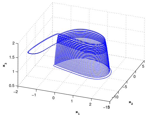
b) (x, y, z) phase portraits of the system (19) with parameters given in (20) with I = 1.5 for r = 0.001
