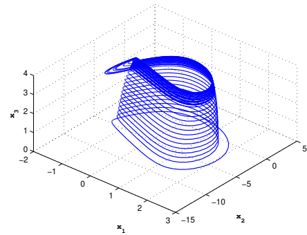
b) (x, y, z) phase portraits of the system (19) with parameters given in (20) and with I = 3.25 for r = 0.008
