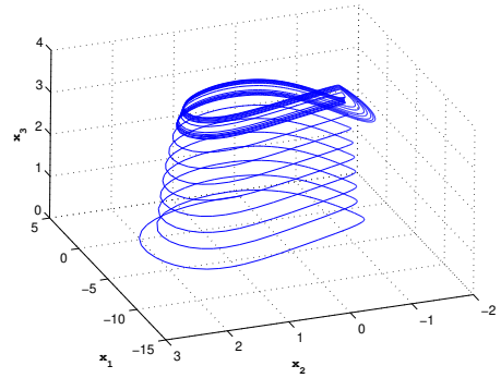
b) (x, y, z) phase portraits of the system (19) with parameters given in (20) and with I = 3.25 for r = 0.0145
