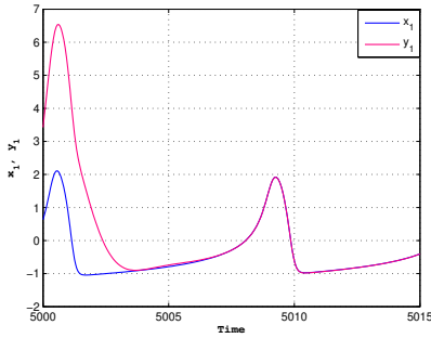
a) synchronization of membrane potential when the injected current in the neuron I = 1 and the ratio of time scales between spiking (fast dynamics) and resting (slow dynamics) r = 0.001
