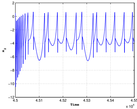
c) Time series portraits of the system (19) with parameters given in (20) and with I = 3.25 for r = 0.0145 , a period doubling cascade is observed
