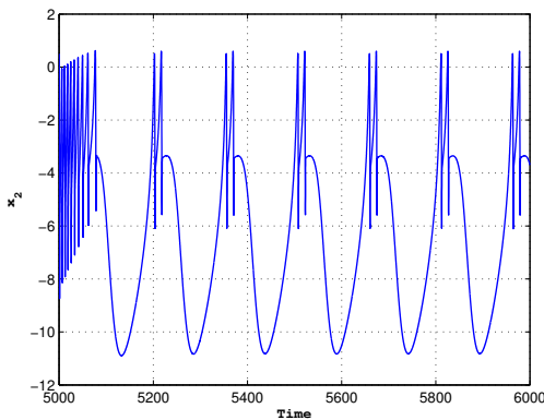
c) Time series portraits of the system (19) with parameters given in (20) with I = 3.25 for r = 0.001 , the neuron behaviour changes from tonic spiking to bursting is observed
