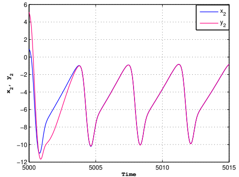
b) synchronization of the exchange of ions across the neuron membrane through fast ionic channels when the injected current in the neuron I = 3.25 and the ratio of time scales between spiking and resting r = 0.001
