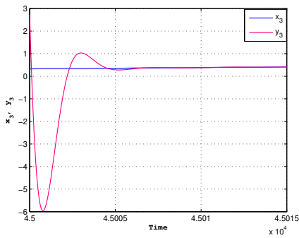
c) synchronization of the exchange of ions through slow ionic channels when the injected current in the neuron I = 2 and the ratio of time scales between spiking and resting r = 0.001
