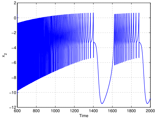
a) Time series portraits of the system (19) with parameters given in (20) with I = 3 for r = 0.001 , a period doubling cascade with a period three solution is observed
