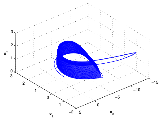
d) (x, y, z) phase portraits of the system (19) with parameters given in (20) with I = 2 for r = 0.001
