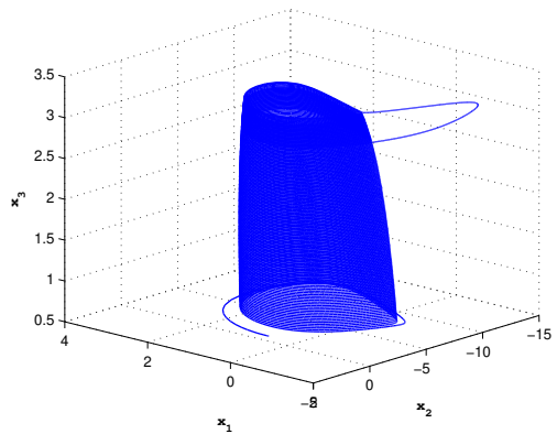
d) (x, y, z) phase portraits of the system (19) with parameters given in (20) with I = 3.25 for r = 0.001
