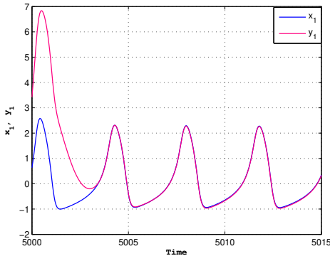
a) synchronization of membrane potential when the injected current in the neuron I = 3.25 and the ratio of time scales between spiking and resting r = 0.001
