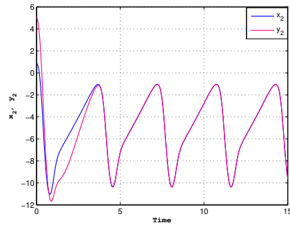
b) synchronization of the exchange of ions across the neuron membrane through fast ionic channels when the injected current in the neuron I = 3.25 and the ratio of time scales between spiking and resting r = 0.0001
