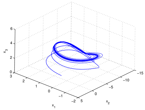
d) (x, y, z) phase portraits of the system (19) with parameters given in (20) and with I = 3.25 for r = 0.05
