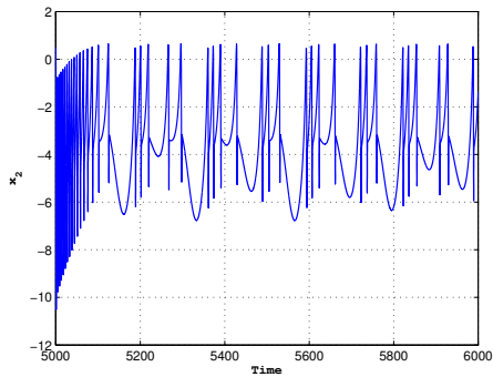
a) Time series portraits of the system (19) with parameters given in (20) and with I = 3.25 for r = 0.008 , a period doubling cascade with a period three solution is observed
