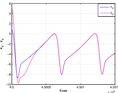
e) synchronization of the exchange of ions across the neuron membrane through fast ionic channels when the injected current in the neuron I = 1.5 and the ratio of time scales between spiking and resting r = 0.001
