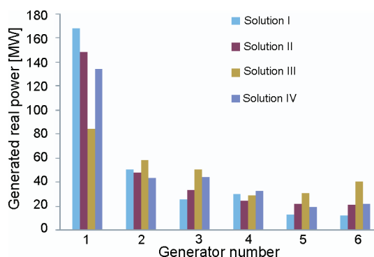
Fig. 3. Control variable setting for corrective action – case B
