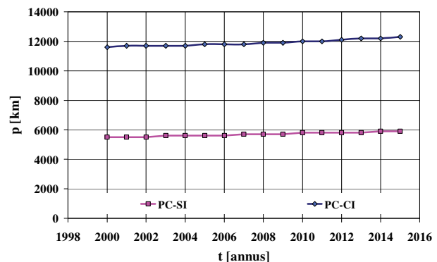
Fig. 2. Annual mileage of passenger cars with spark ignition- and compression ignition engines
