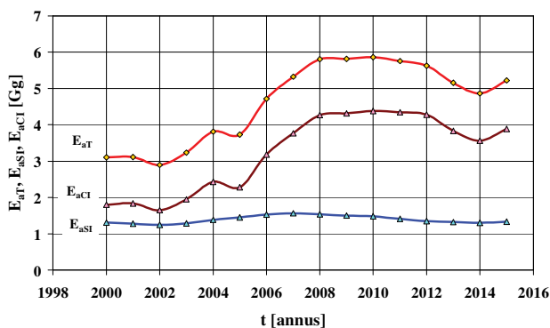
Fig. 13. National annual emission of particulate matter PM10 from tribological elements of passenger cars
