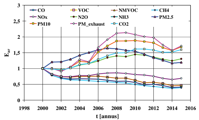
Fig. 16. Relative national annual emission of individual pollutants
