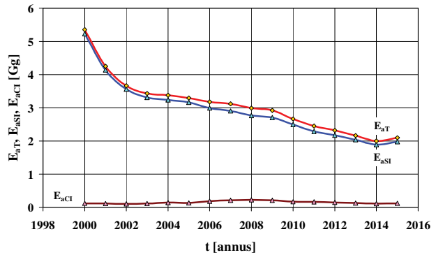
Fig. 8. National annual emission of methane from passenger cars
