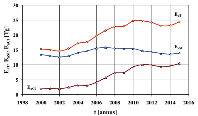
Fig. 15. National annual emission of carbon dioxide from passenger cars
