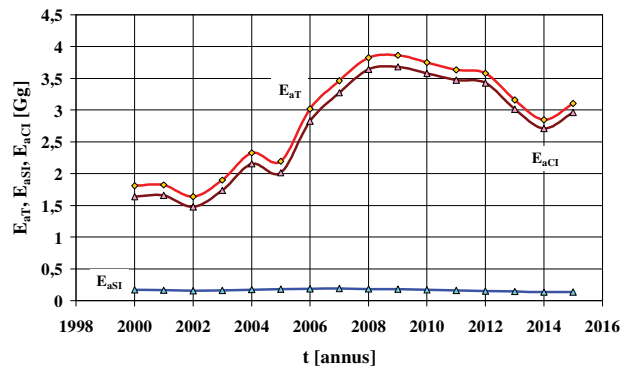
Fig. 14. National annual emission of particulate matter from the exhaust system of passenger car engines
