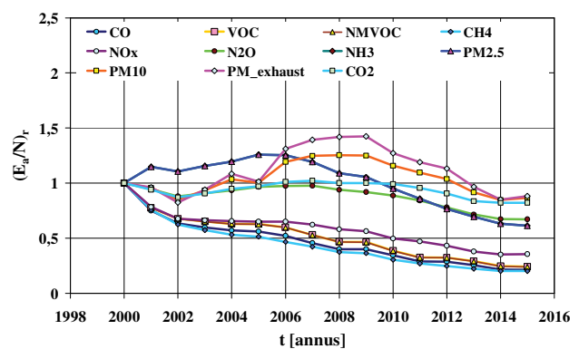
Fig. 17. Relative national annual emission of individual pollutants from a single passenger car
