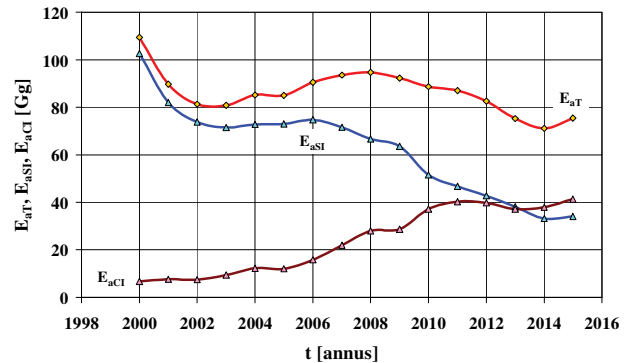
Fig. 9. National annual emission of nitrogen oxides from passenger cars
