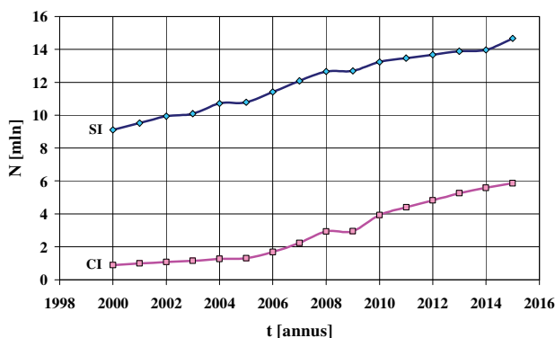
Fig. 1. Number of passenger cars with spark ignition- and compression ignition engines
