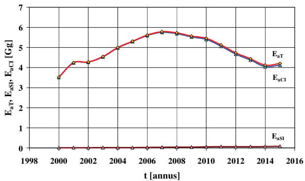
Fig. 11. National annual emission of ammonia from passenger cars
