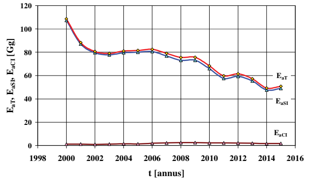
Fig. 6. National annual emission of volatile organic compounds from passenger cars
