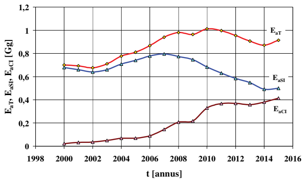
Fig. 10. National annual emission of nitrous oxide from passenger cars
