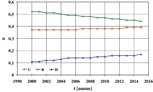
Fig. 3. Mileage of passenger cars under the following model traffic conditions: urban, rural and on highways and expressways
