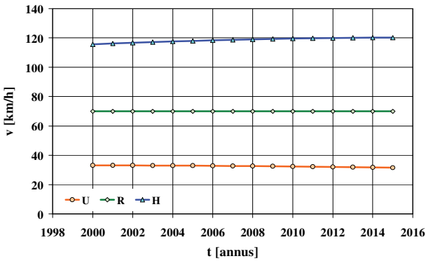
Fig. 4. Average velocity of passenger cars in towns, outside towns, on highways and expressways
