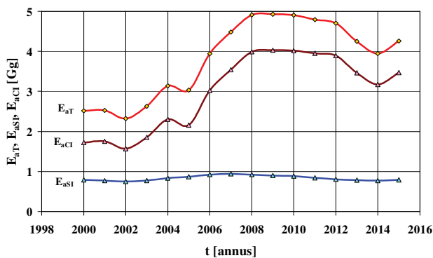
Fig. 12. National annual emission of particulate matter PM2.5 from tribological elements of passenger cars
