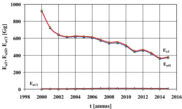
Fig. 5. National annual emission of carbon monoxide from passenger cars
