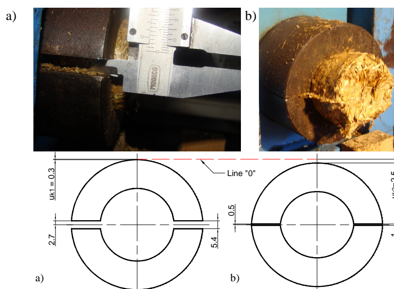
Fig. 5. The value of the gap between the lower and the upper part of the sleeve for an unloading cycle (a) and working cycle (b) during straw briquetting
