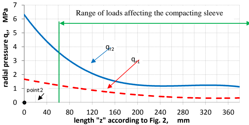
Fig. 3. Diagrams describing the distribution of radial pressures (lateral pressures) q_r in the function of the sleeve length
