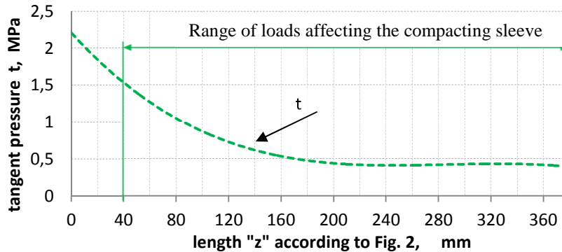
Fig. 4. Diagram of tangent pressure t in the function of the sleeve length
