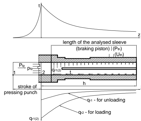
Fig. 2. Scheme of loads within the sleeve Source: Author's research based on pos. [4].
