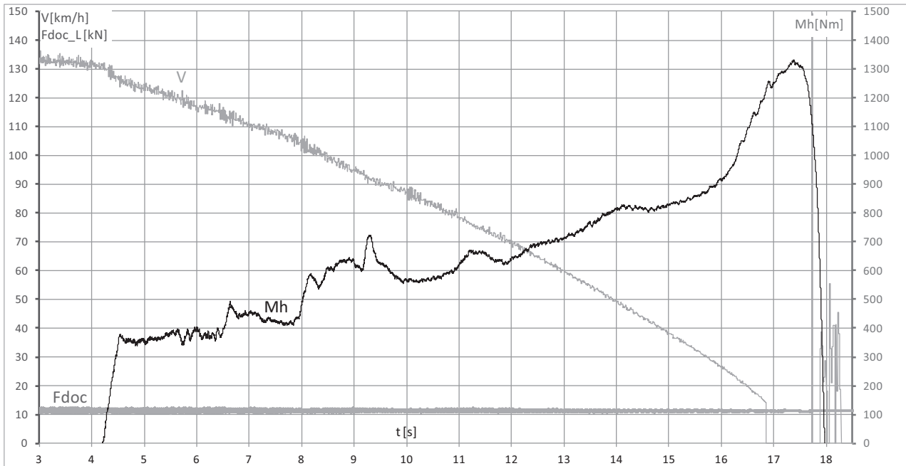
Fig. 9. Test 225, ABS-off, slippery surface, pushing force 11 kN
