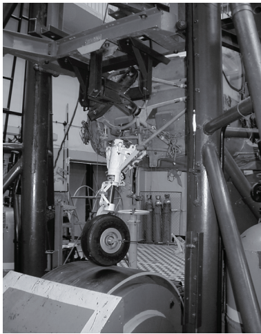
Fig. 4. M3T test stand for full scale brake testing with mounted airplane landing gear (source: IoA)
