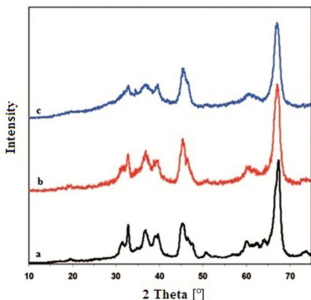
Figure 3. XRD patterns after being calcined at 1000°C for 2 hrs: (a) \gamma - \text{Al}_2\text{O}_3 , (b) 2% wt \text{BaO}/\text{Al}_2\text{O}_3 , and (c) 6% wt \text{BaO}/\text{Al}_2\text{O}_3
