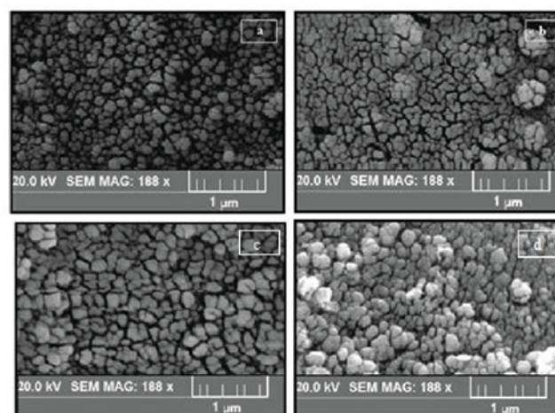
Figure 4. Micrographs of \text{Ir}/\text{BaO}/\gamma - \text{Al}_2\text{O}_3 and \text{Ir}/\gamma - \text{Al}_2\text{O}_3 catalysts a, c) before, and b, d) after being heated at 1000°C for 2 hrs
