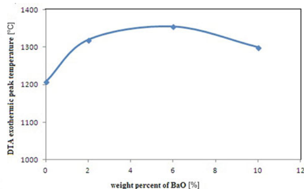
Figure 1. Relationship between the DTA exothermic peak temperature of the \gamma -to- \alpha phase transition and weight percent of barium oxide
