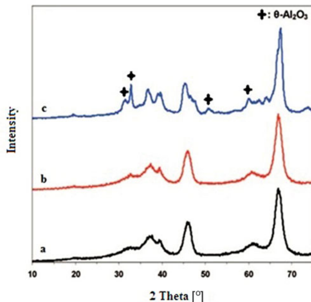
Figure 2. XRD patterns of \gamma - \text{Al}_2\text{O}_3 samples calcined for 2 hrs at (a) 600°C, (b) 800°C, and (c) 1000°C
