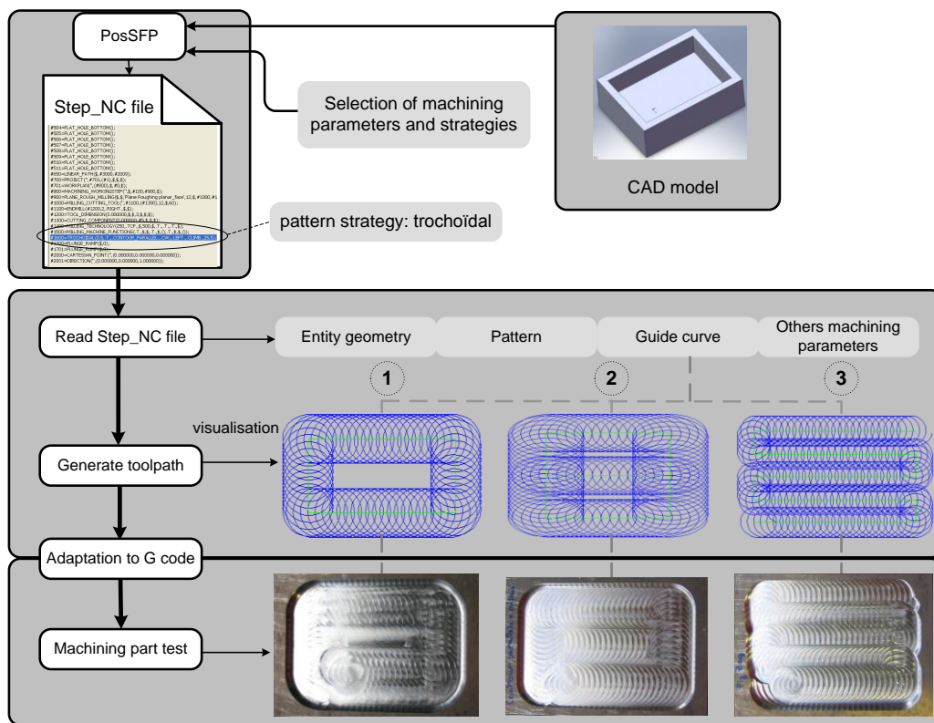
Fig. 6. Trochoidal toolpaths built on pattern strategy in Step_NC numerical chain
