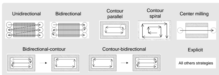
Fig. 1. Strategies proposed in Step_NC norms
