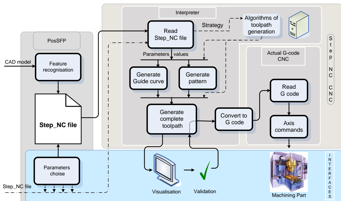
Fig. 5. Step_NC numerical chain to generate pattern toolpaths
