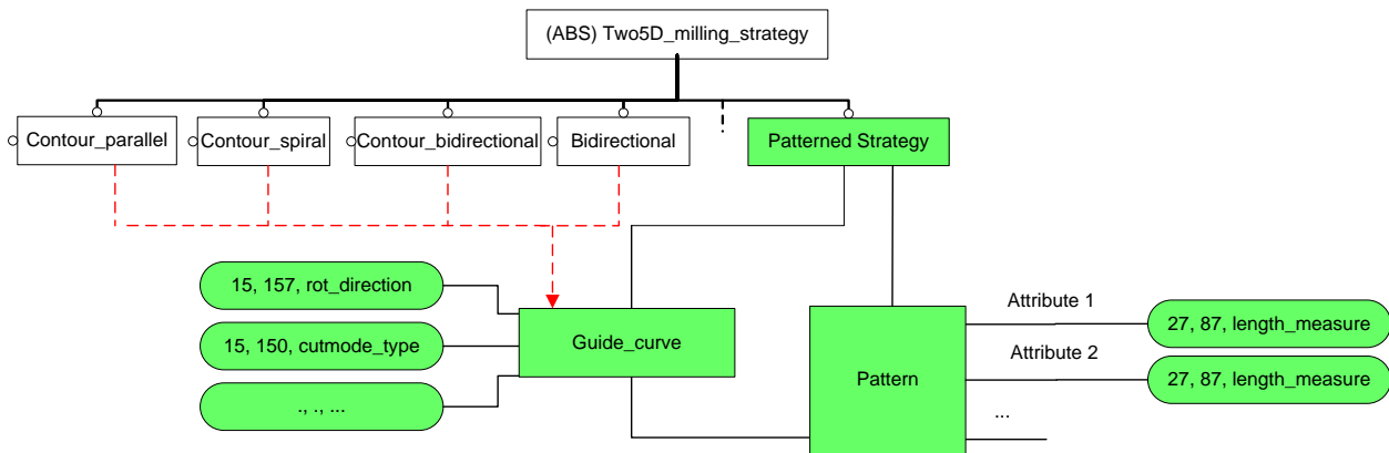
Fig. 3. ARM diagram completed with pattern strategies
