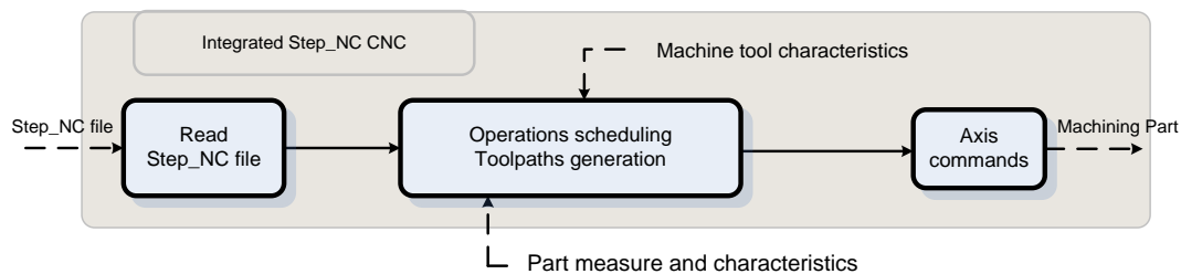
Fig. 8. Integrated Step_NC programming
