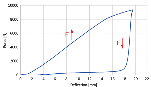
Fig. 5. Force / deflection diagram of the contact strip F20E10 Cu40 type [own work]
