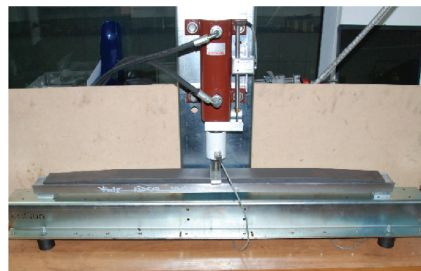
Fig. 2. The view of the stand to determine the deflection of characteristic of the contact strip [photo. K. Franczak]
