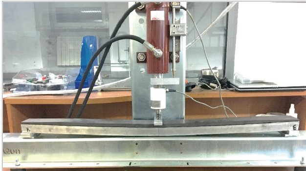
Fig. 6. The view of the contact strip under a load of 9.3 kN [photo. K. Franczak]
