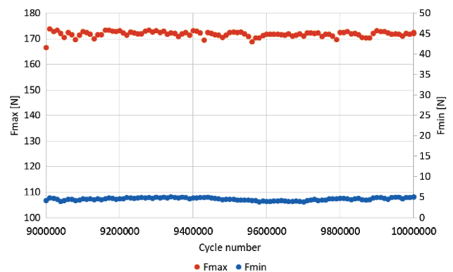
Fig. 10. The example of the second part of the mechanical fatigue resistance of the carbon contact strip (9–10 million cycles) [own work]
