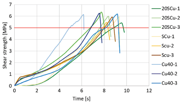
Fig. 7. The results of the conducted shear strengths tests of contact strips (3 samples of each type) in room temperature (20°C) [own work]
