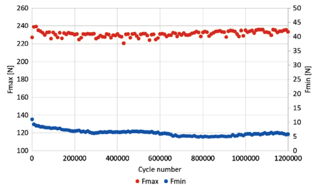
Fig. 9. The diagram of the first part of the mechanical fatigue resistance of the carbon contact strip (1,2 million cycles) [own work]
