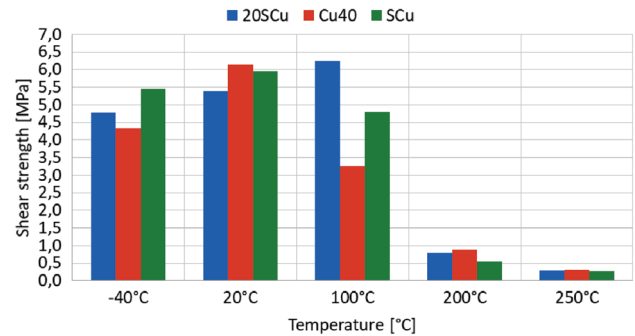
Fig. 8. The results of the shear strengths tests of the carbon contact strips in various temperatures [own work]
