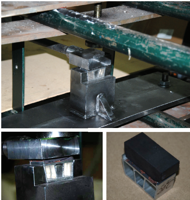
Fig. 3. The view of the test stand for shear strength research of the contact strips [photo. K. Franczak]
