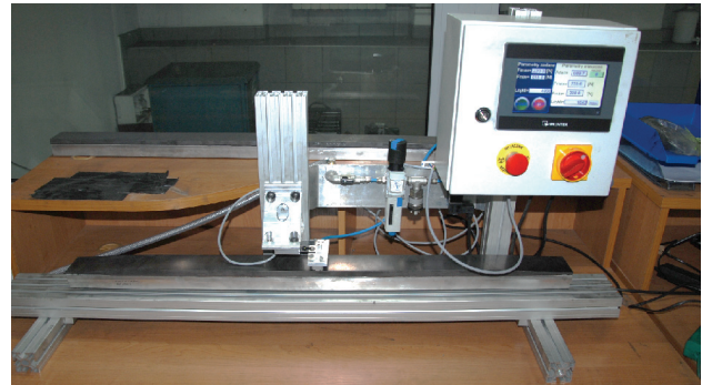
Fig. 4. The view of the specialist fatigue testing device for contact strips [photo. K. Franczak]
