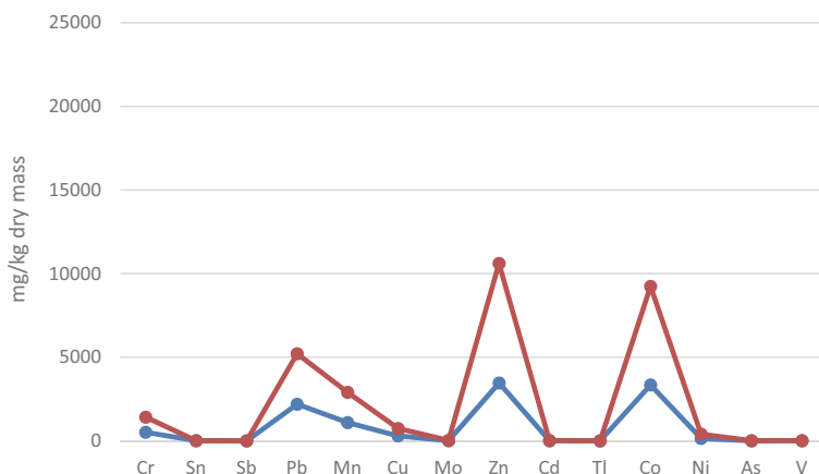
Fig. 2. Results of elements contents in 2 samples of large-sized waste ash tests
