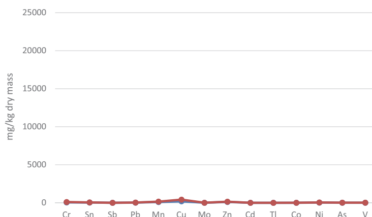
Fig. 5. Results of elements contents in 2 samples of paper waste ash tests
