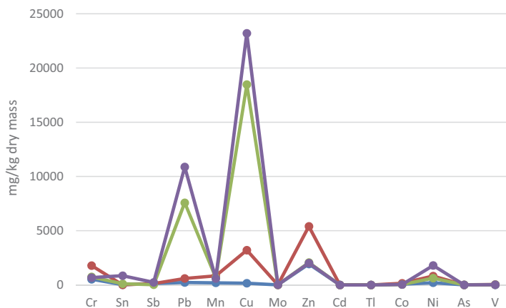
Fig. 3. Results of elements contents in 4 samples of plastic waste ash tests
