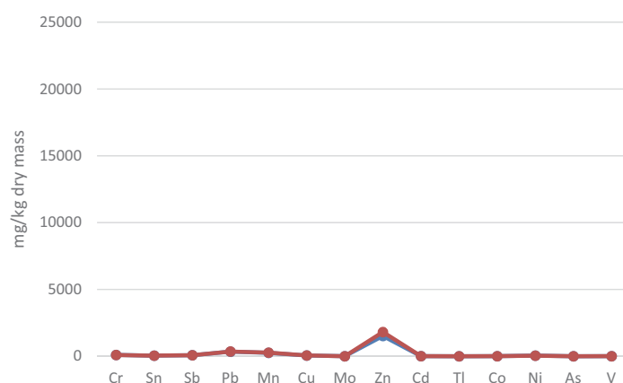
Fig. 6. Results of elements contents in 2 samples of textile waste ash tests
