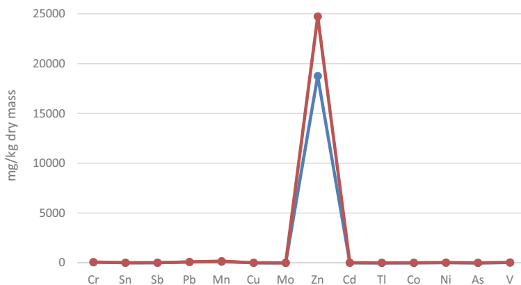
Fig. 4. Results of elements contents in 2 samples of rubber waste ash tests
