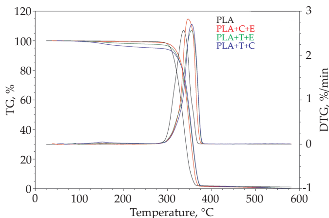
Fig. 2. TG curves for sample non-modified and modified with biocidal agents
