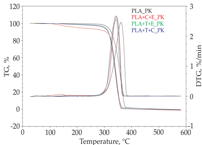
Fig. 5. TG curves for degraded samples
