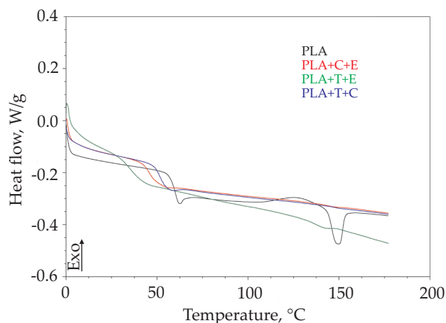
Fig. 1. DSC curves for samples non-modified and modified with biocidal agents
