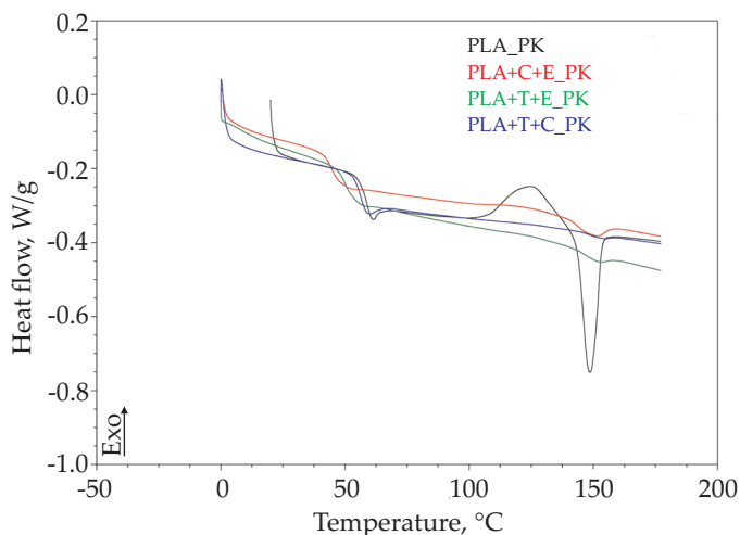
Fig. 4. DSC curves for degraded samples
