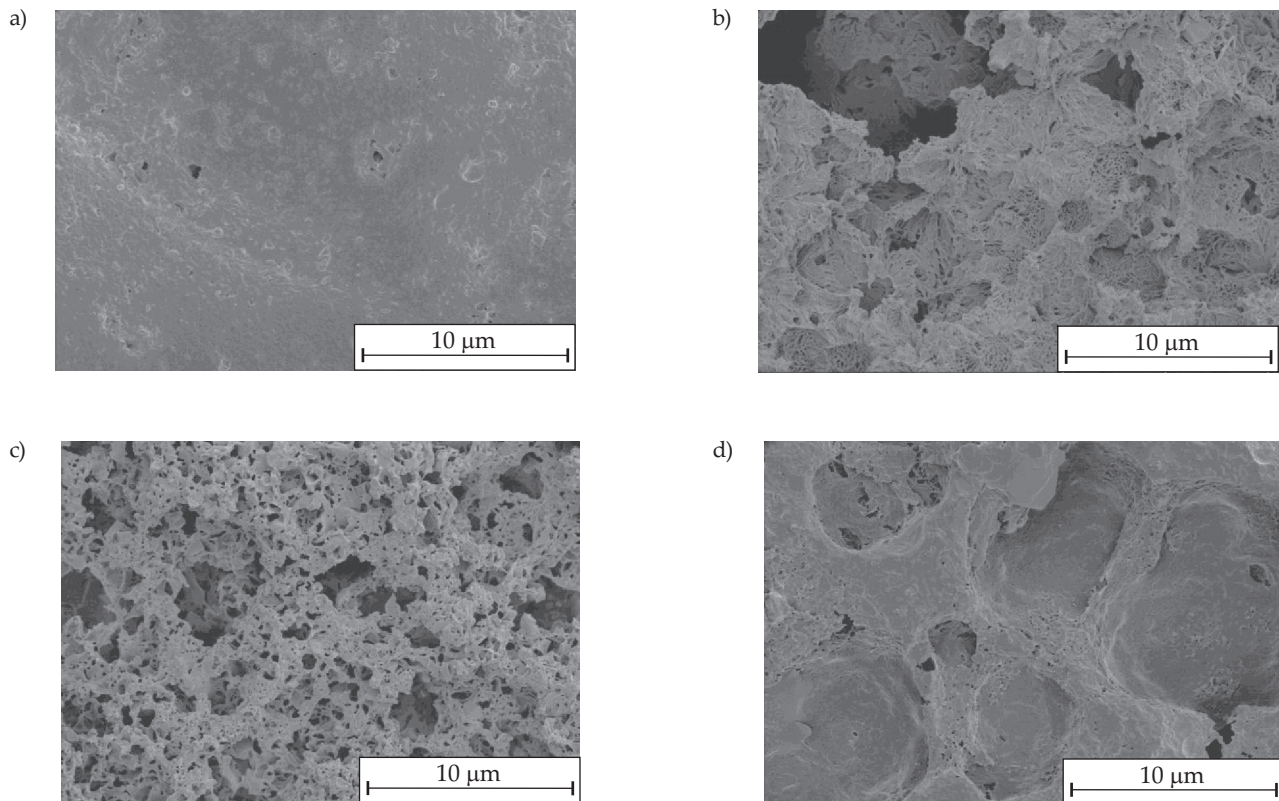
Fig. 7. SEM images of PLA samples subjected to degradation in proteinase K for 7 weeks: a) PLA_PK, b) PLA+C+E_PK, c) PLA+T+E_PK, d) PLA+T+C_PK
