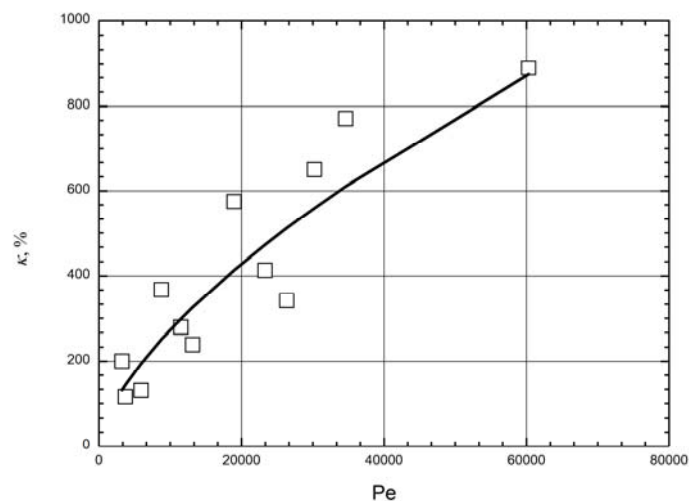
Fig. 7. A comparison of the obtained results for the tested static mixer and an empty pipe
