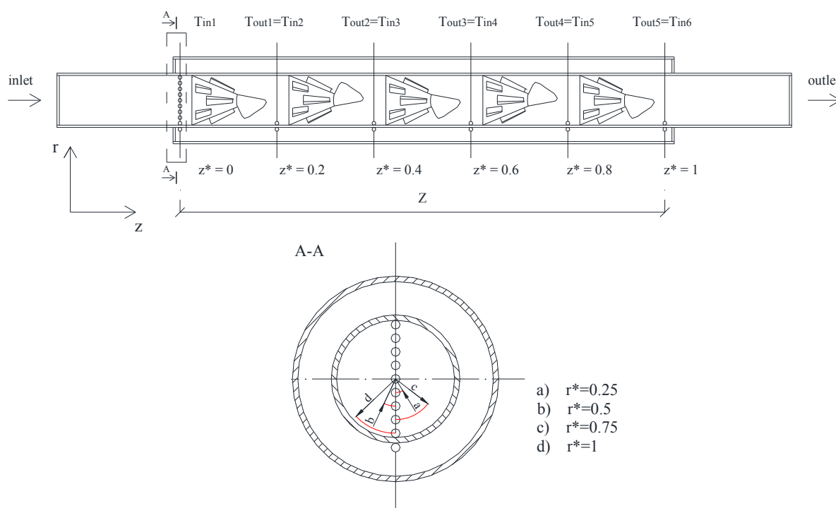
Fig. 2. The thermal probe positions in the experimental set-up
