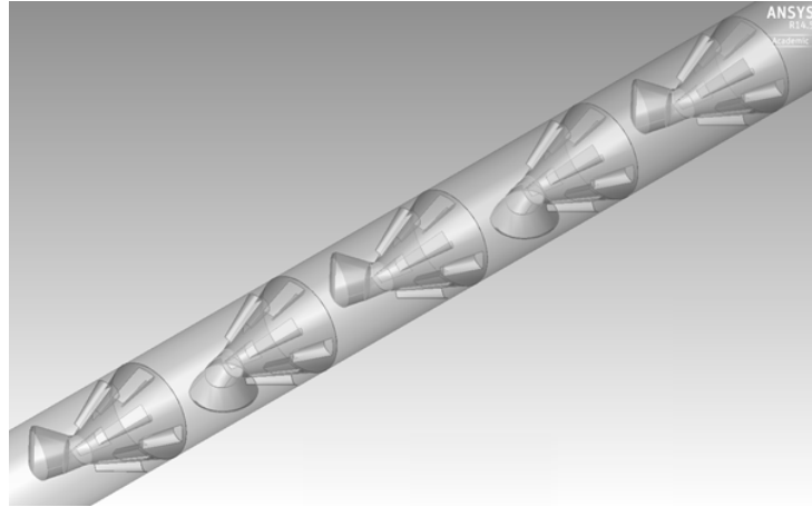
Fig. 3. View of geometry used in CFD simulations
