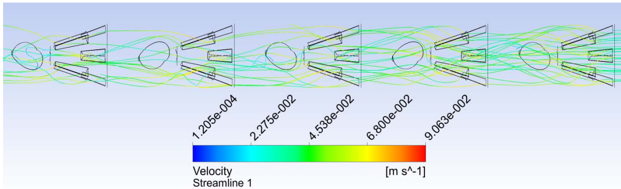
Fig. 9. The typical streamline of fluid velocity (water, \dot{m} = 0.28 \text{ kg s}^{-1} )
