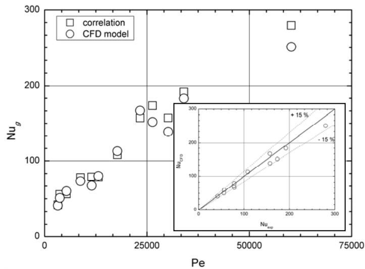
Fig. 10. Comparison of predicted (CFD model) and correlated (calculated values) global Nusselt numbers as the function of the dimensionless Péclet number
