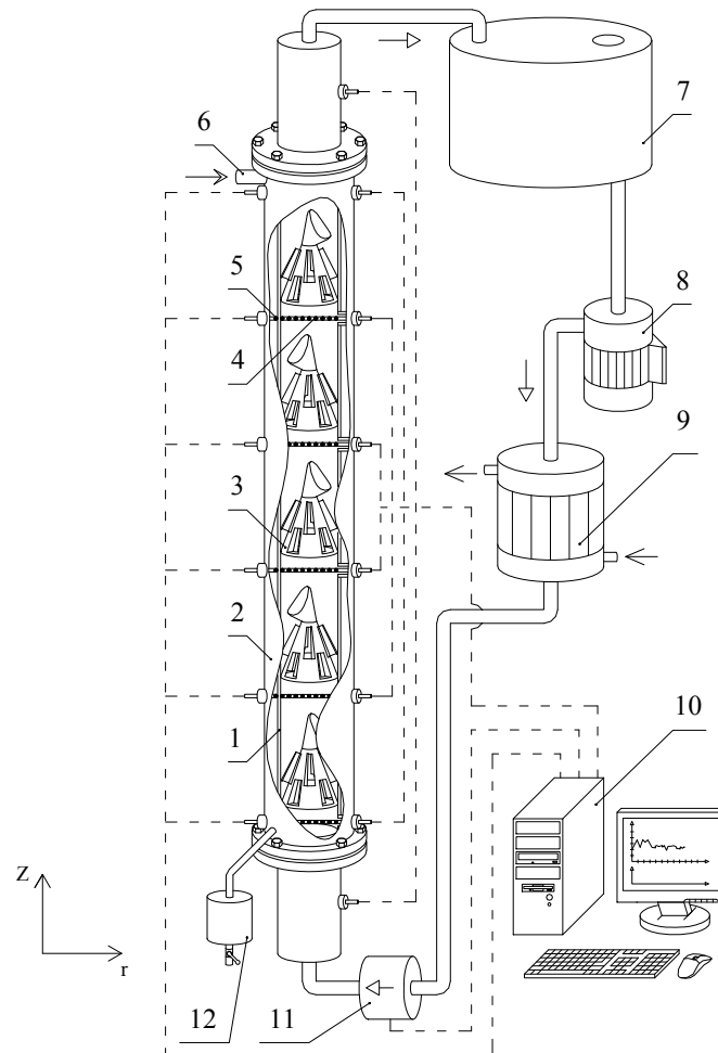
Fig. 1. The sketch of experimental set-up: 1 - wall, 2 - heat jacket, 3 - insert, 4 - internal temperature sensors, 5 - wall temperature sensor, 6 - steam inlet, 7 - buffer, 8 - circulation pump, 9 - heat exchanger, 10 - personal computer, 11 - flow meter, 12 - condensate outlet
