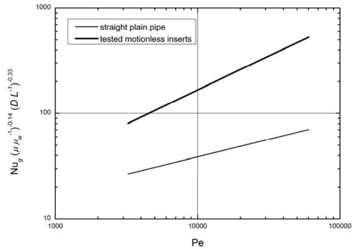
Fig. 6. A comparison of the obtained results for the tested static mixer and an empty pipe
