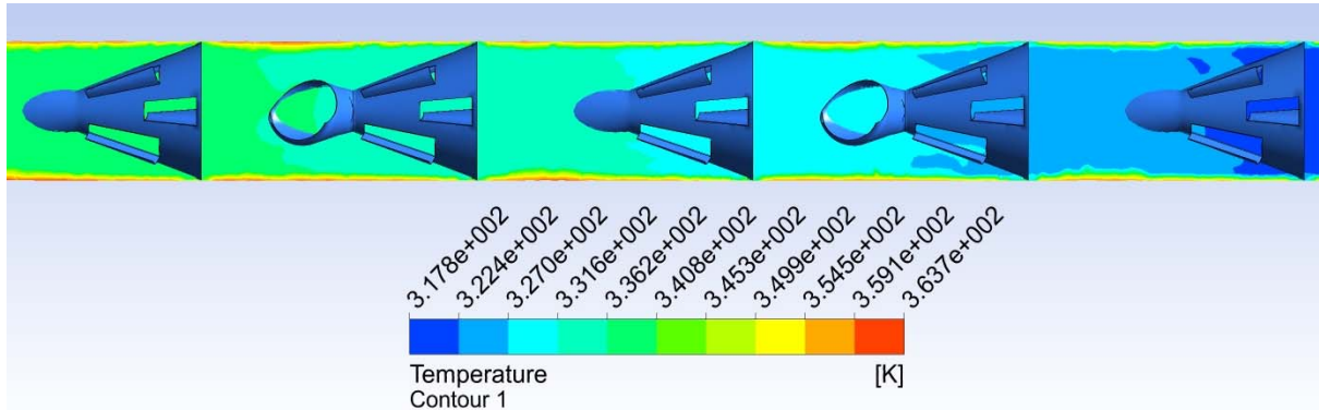
Fig. 8. The temperature contour generated by CFD modelling (water, \dot{m} = 0.04 \text{ kg s}^{-1} )
