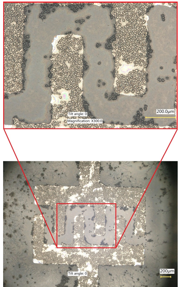
Fig. 5. The dead cells on one of the electrodes after the experiment
