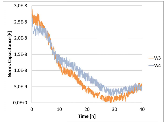
Fig. 4. Capacitance response measured by an ECIS sensor array with NiCr electrode at 64 kHz
