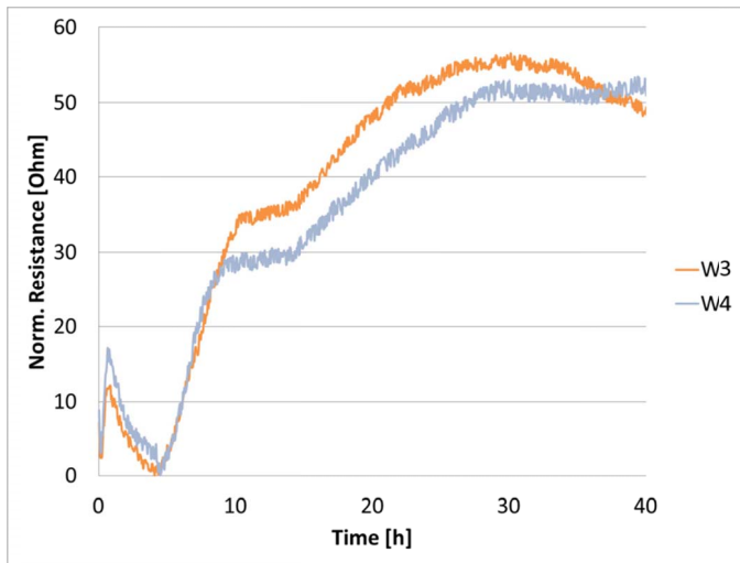
Fig. 3. Resistance response measured by an ECIS sensor array with NiCr electrode at 62.5 Hz
