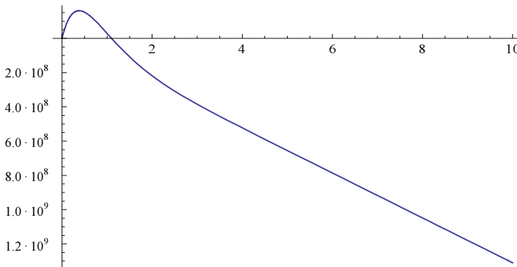
Fig. 1. Income chart v_2(2, 2, t) on interval [0, 10]
