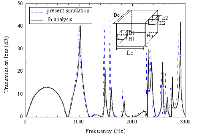
Fig. 5. Comparison of the simulated results of a concentric straight expansion chamber muffler with Ih's analytic solution (muffler A: B_o=H_o=0.15 m, B_1=B_2=H_1=H_2=0.05 m, L_o=0.025 m) (IH, 1992).
