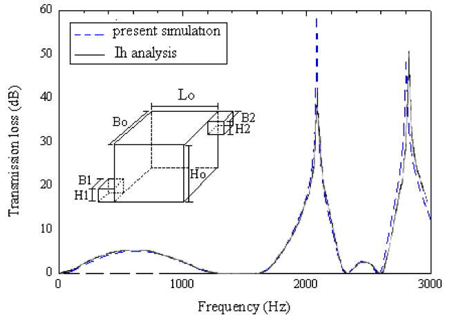
Fig. 6. Comparison of the simulated results of a bias straight expansion chamber muffler with Ih's analytic solution (muffler B: B_o=H_o=0.15 m, B_1=B_2=H_1=H_2=0.05 m, L_o=0.025 m) (IH, 1992).
